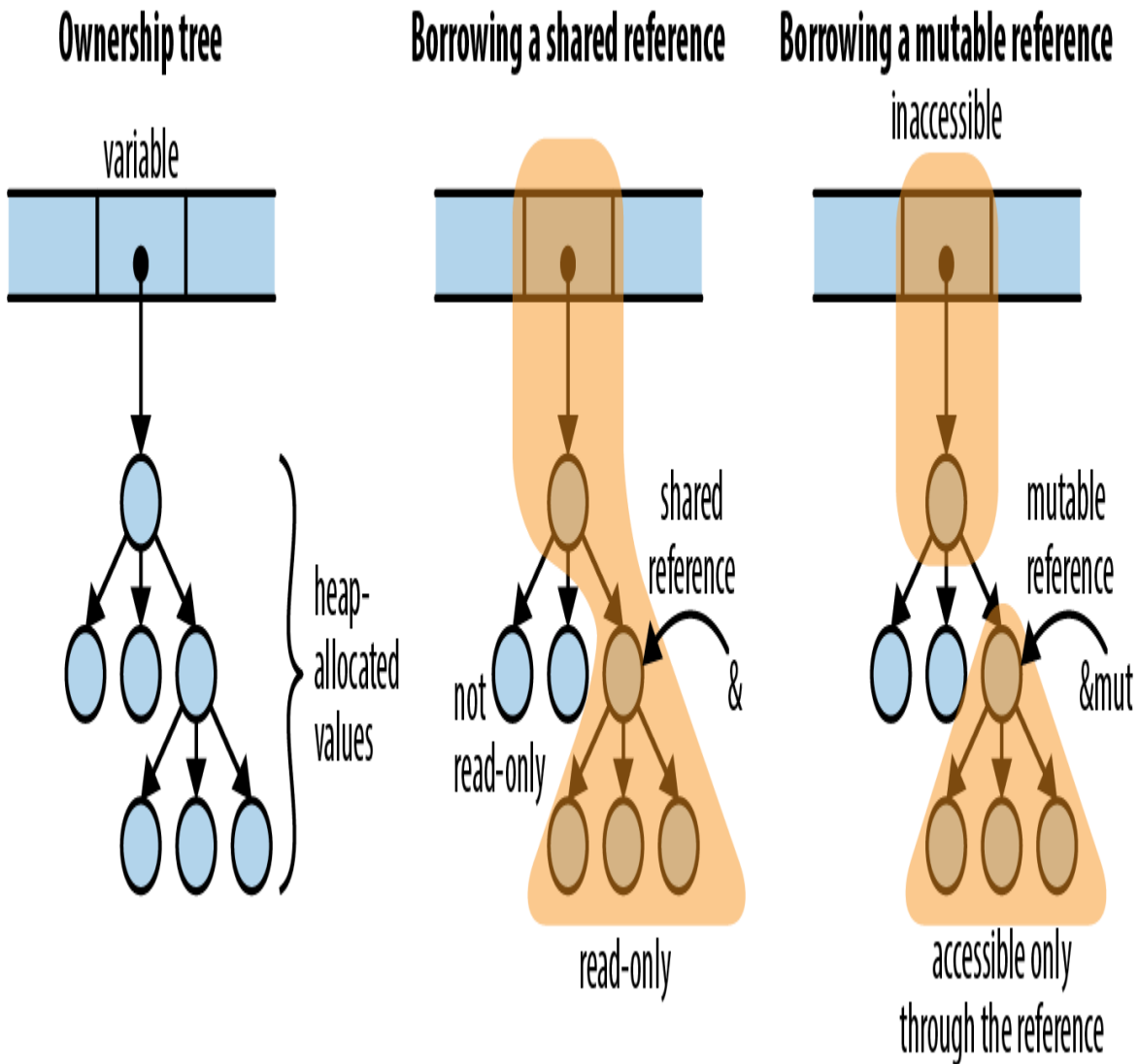
Figure 5-9. Borrowing a reference affects what you can do with other values in the same ownership tree
