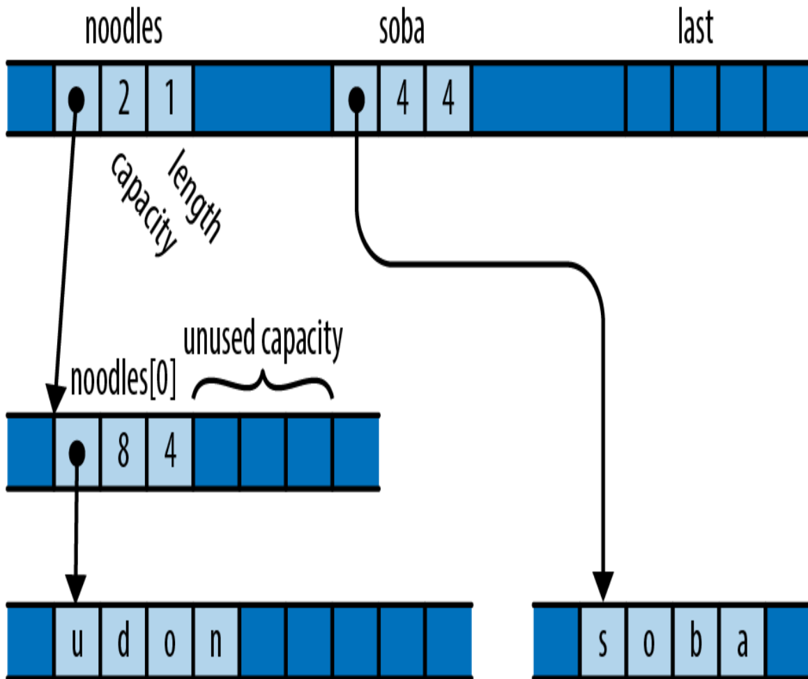
Figure 22-3. A vector with uninitialized, spare capacity
