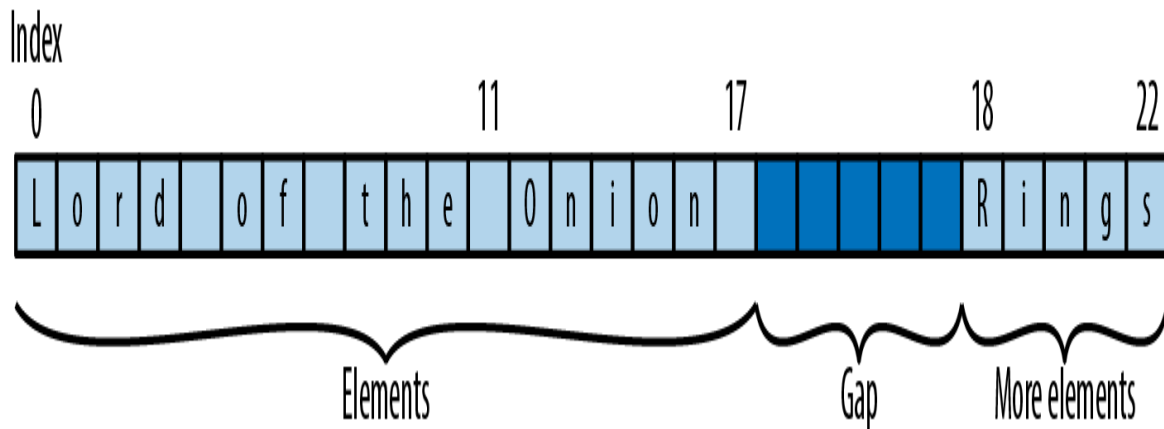
Figure 22-7. A gap buffer containing some more text
