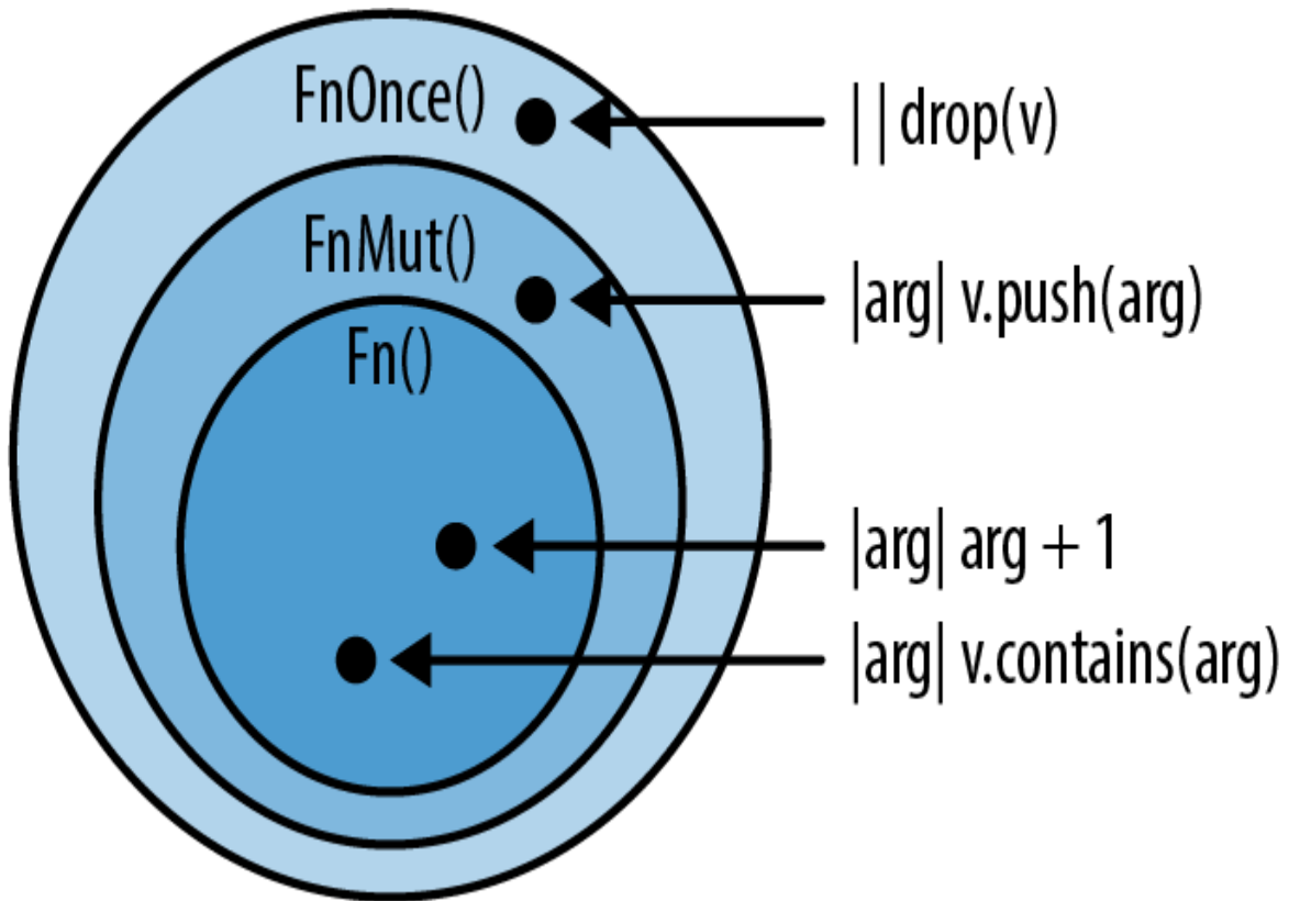
Figure 14-2. Venn diagram of the three closure categories
