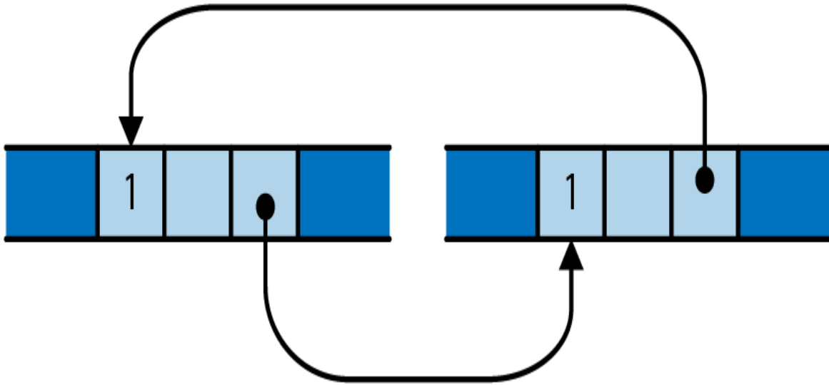
Figure 4-13. A reference-counting loop; these objects will not be freed
