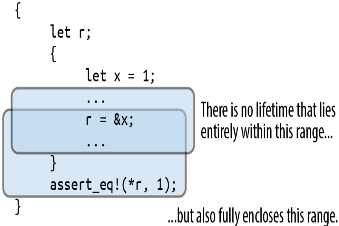
Figure 5-5. A reference with contradictory constraints on its lifetime
