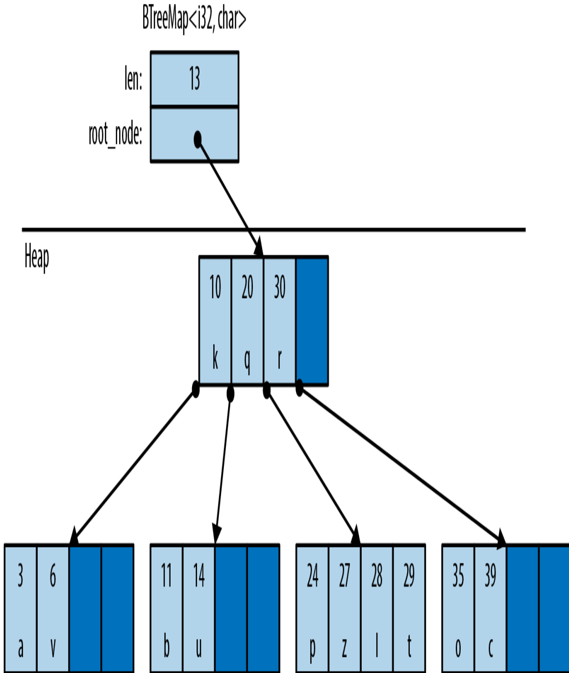
Figure 16-5. A BTreeMap in memory
