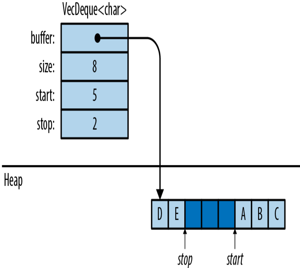
Figure 16-3. How a VecDeque is stored in memory
