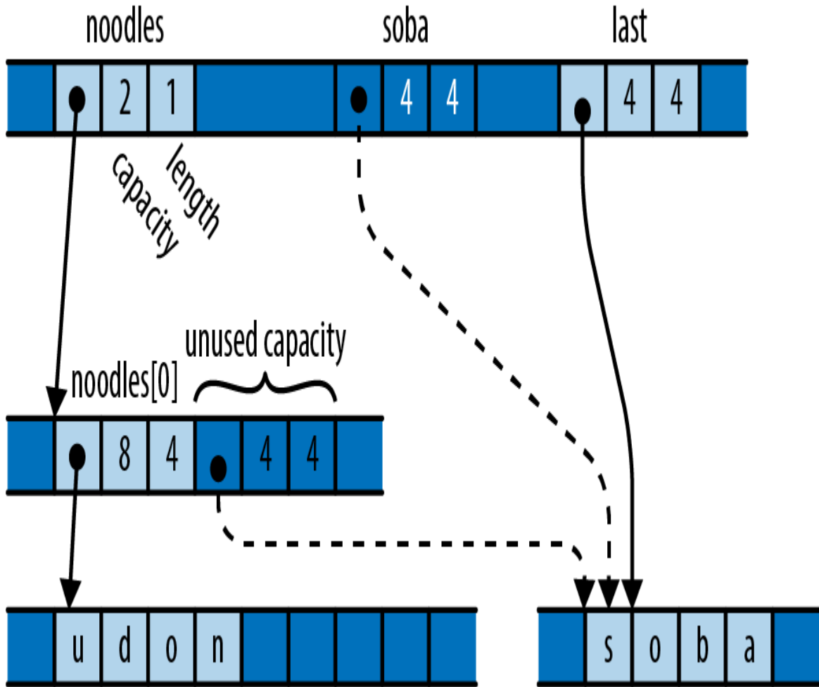
Figure 22-5. After popping an element from the vector into last
