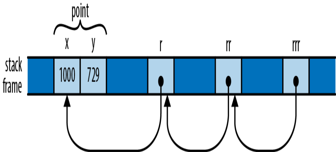
Figure 5-2. A chain of references to references
