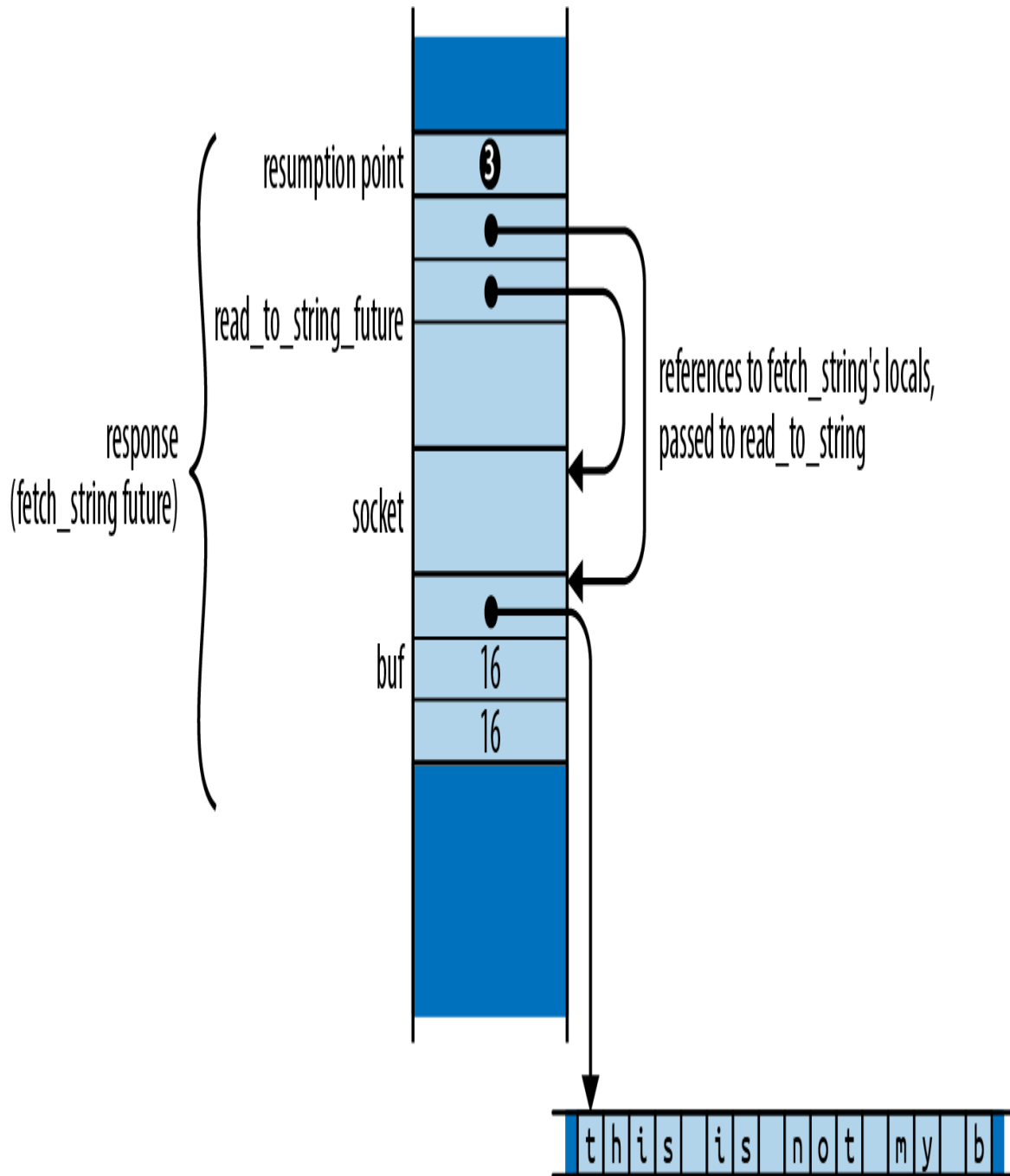
Figure 20-6. The same future, in the midst of awaiting read_to_string
