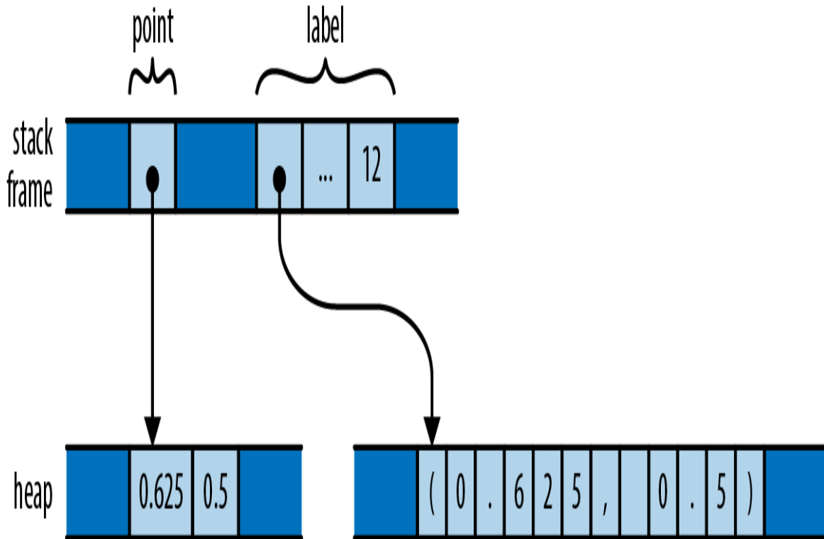
Figure 4-3. Two local variables, each owning memory in the heap
