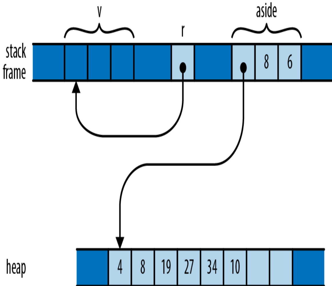
Figure 5-7. A reference to a vector that has been moved away
