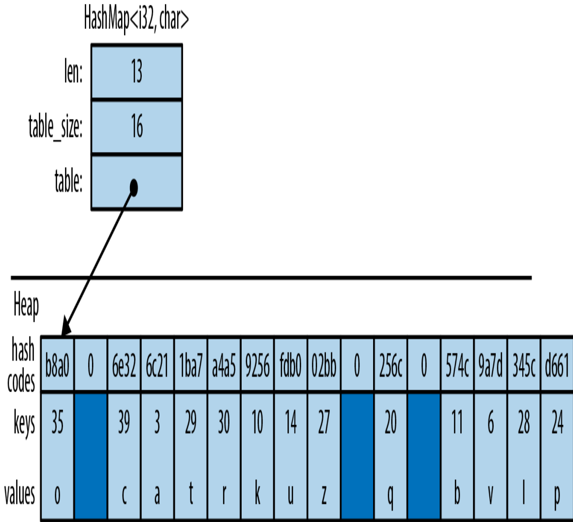
Figure 16-4. A HashMap in memory
