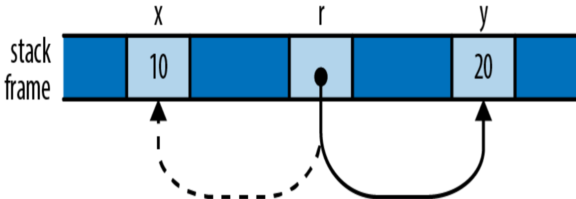
Figure 5-1. The reference r , now pointing to y instead of x
