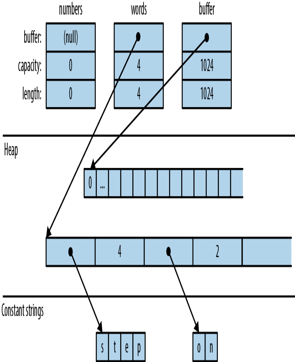
Figure 16-1. Vector layout in memory: each element of words is a &str value consisting of a pointer and a length
