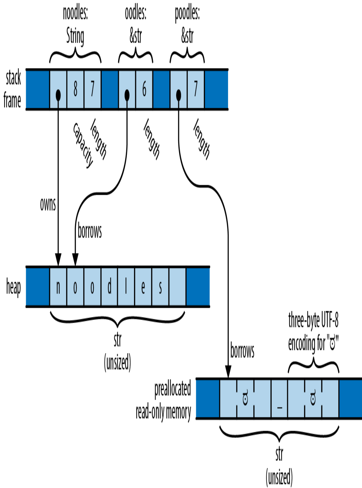
Figure 3-3. String , &str , and str
