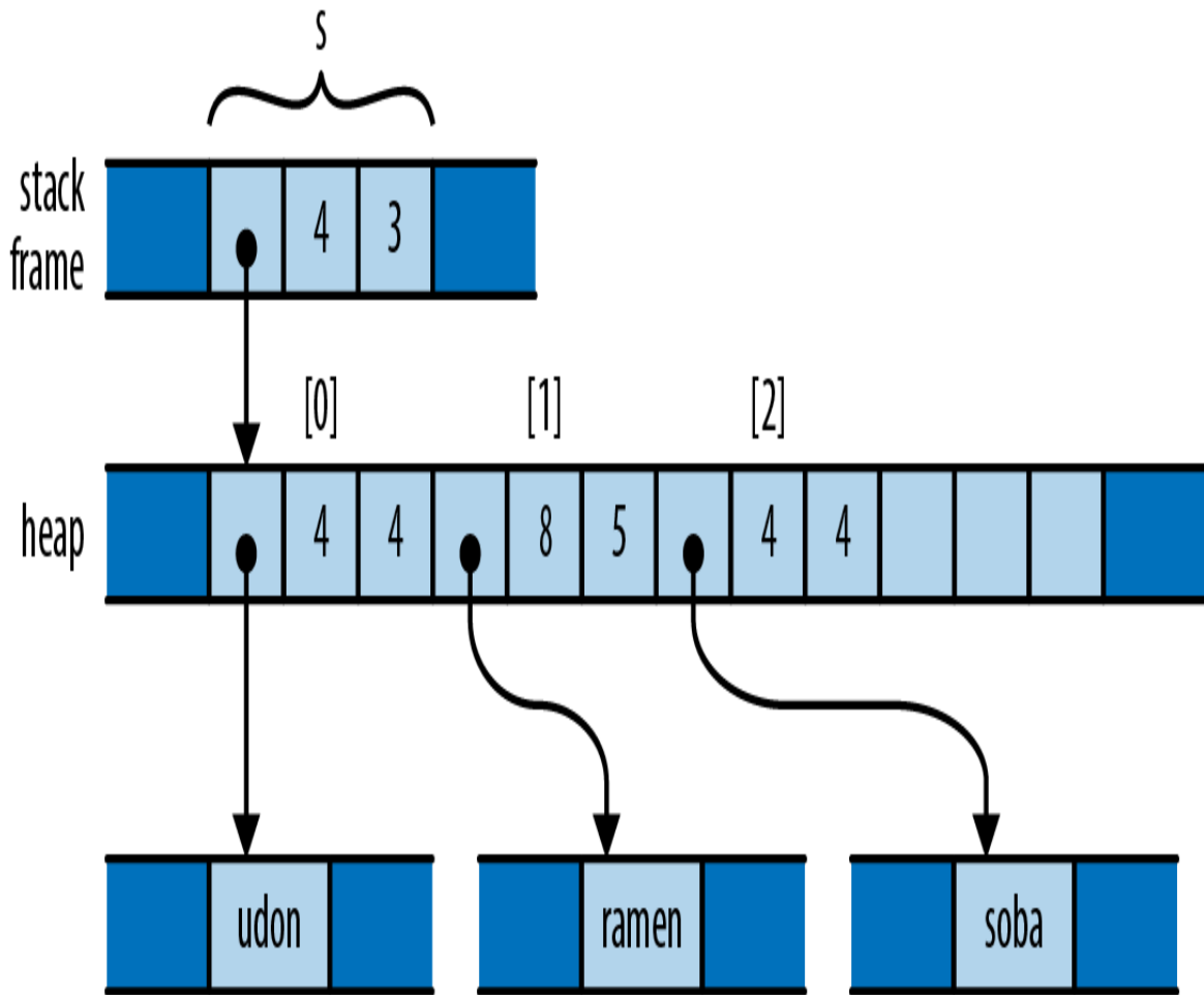
Figure 4-7. How C++ represents a vector of strings in memory
