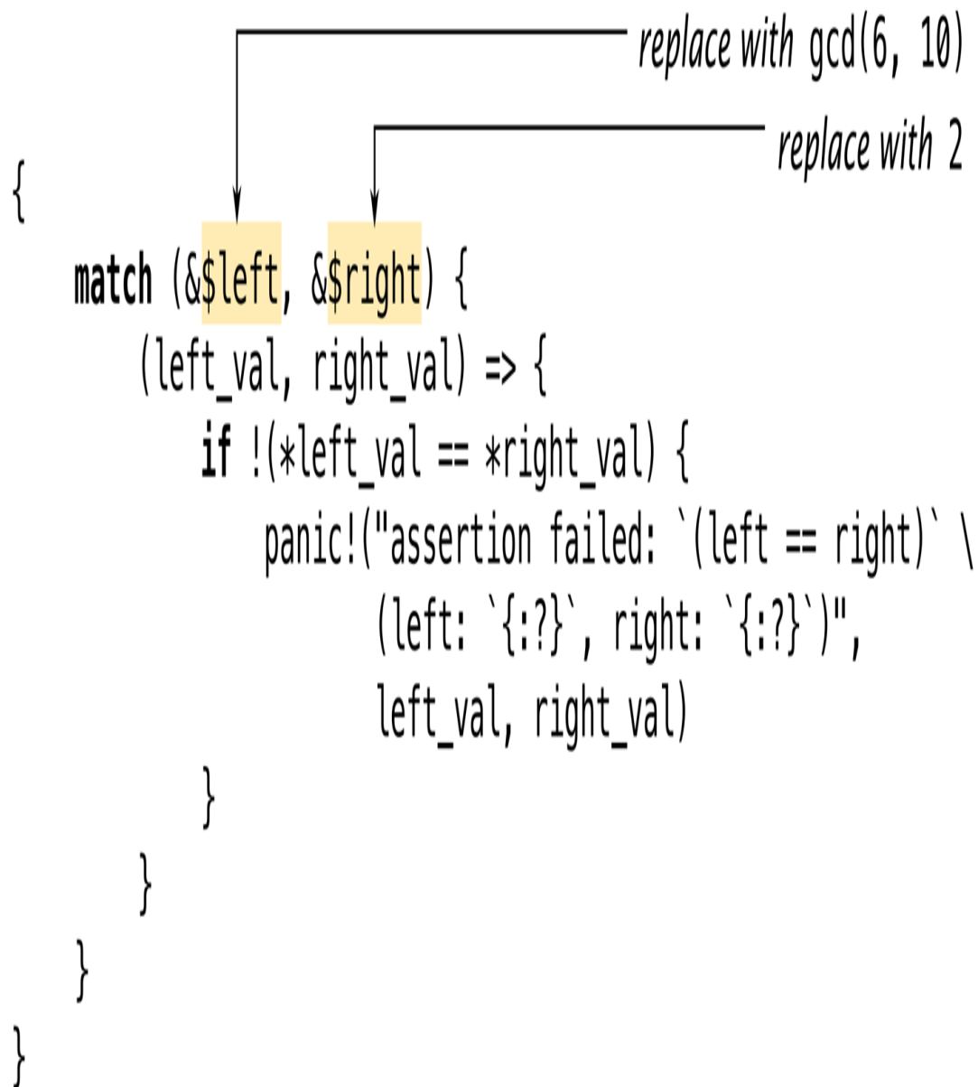
Figure 21-3. Expanding a macro, part 2: filling in the template
