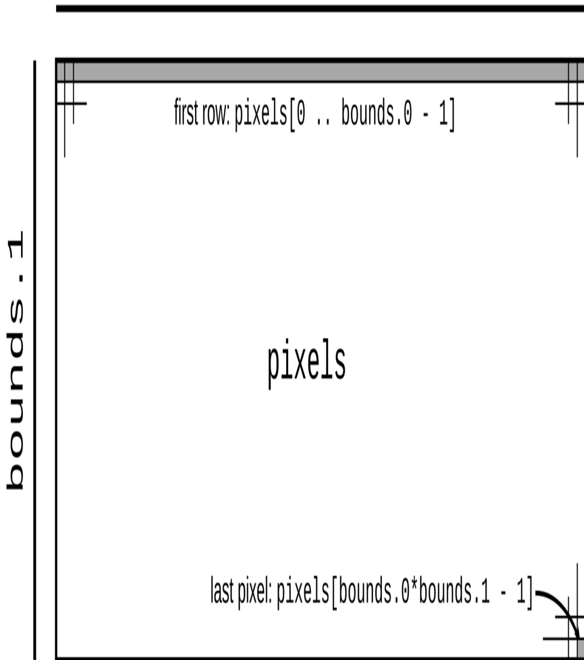
Figure 2-5. Using a vector as a rectangular array of pixels
