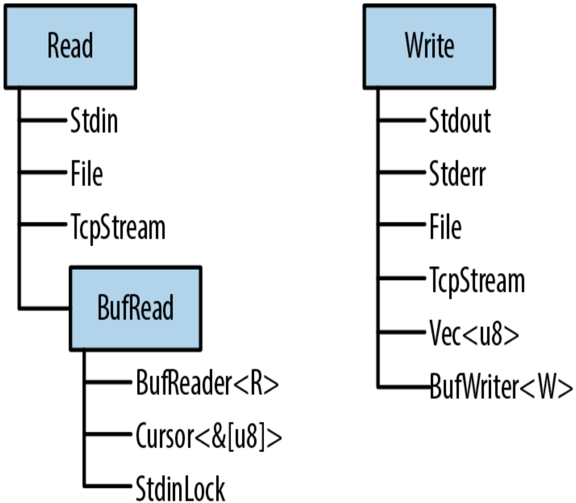
Figure 18-1. Rust's three main I/O traits and selected types that implement them
