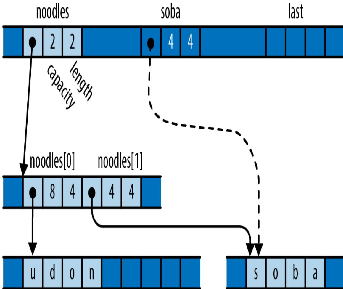
Figure 22-4. After pushing soba 's value onto the vector
