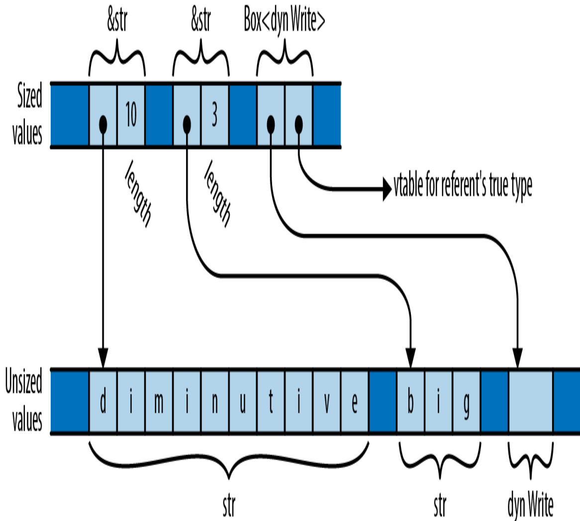
Figure 13-1. References to unsized values
