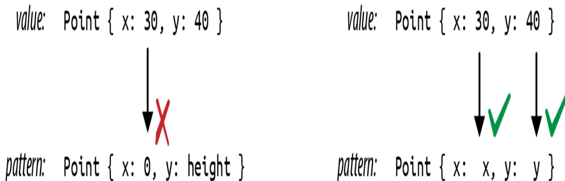
Figure 10-6. Pattern matching with structs
