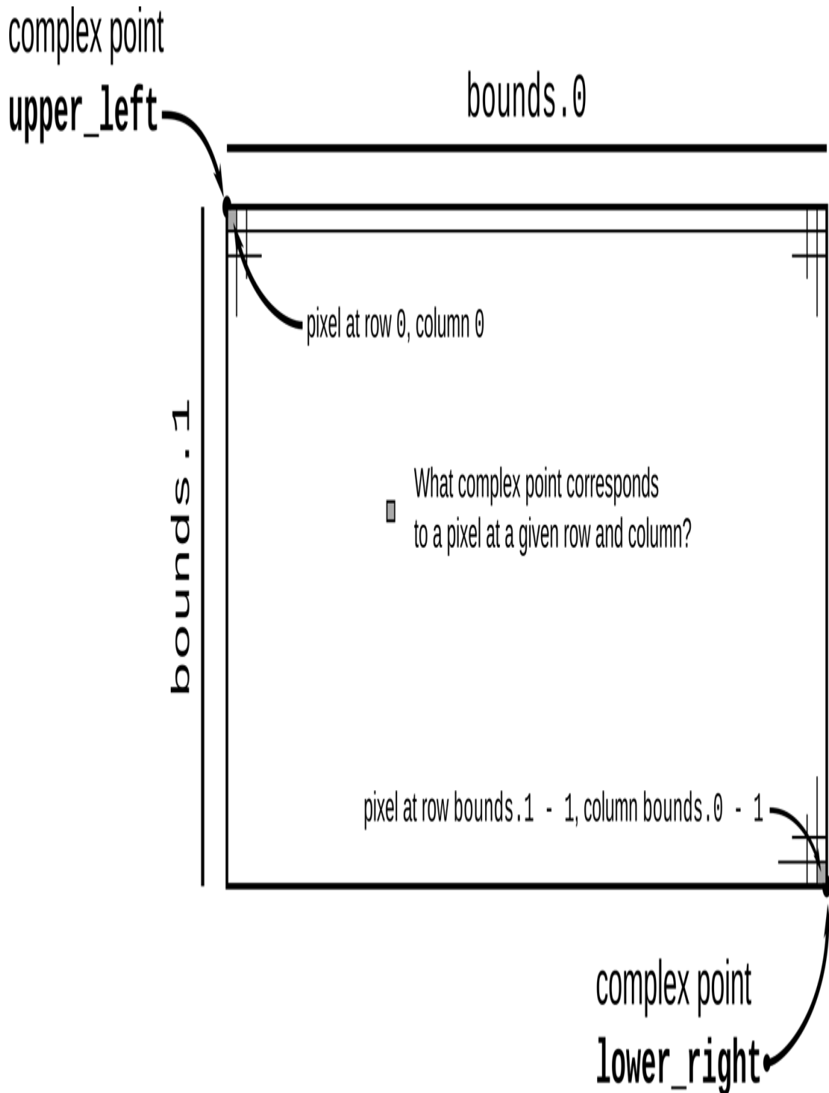
Figure 2-4. The relationship between the complex plane and the image's pixels
