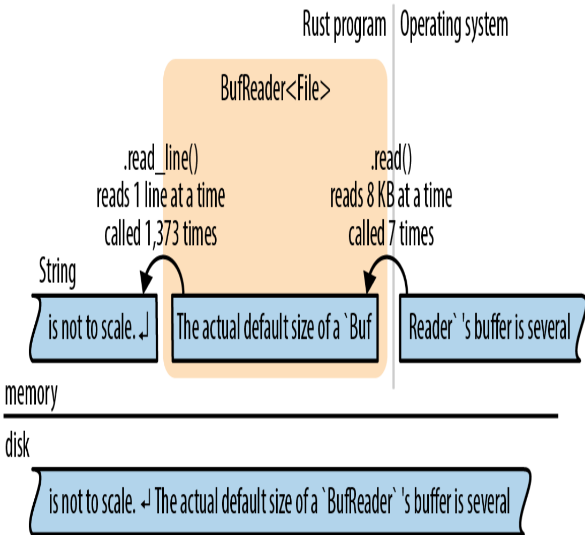
Figure 18-2. A buffered file reader
