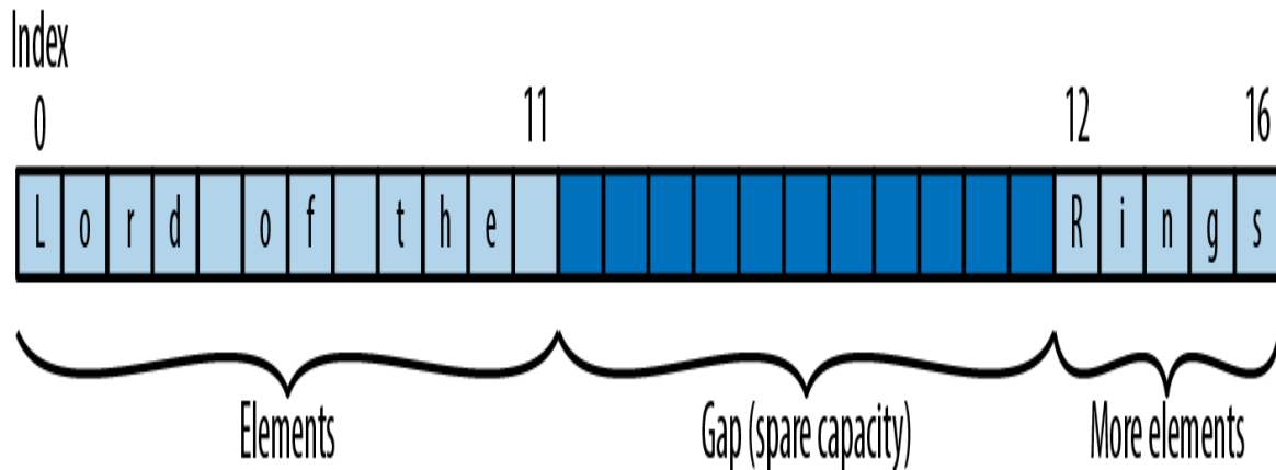
Figure 22-6. A gap buffer containing some text
