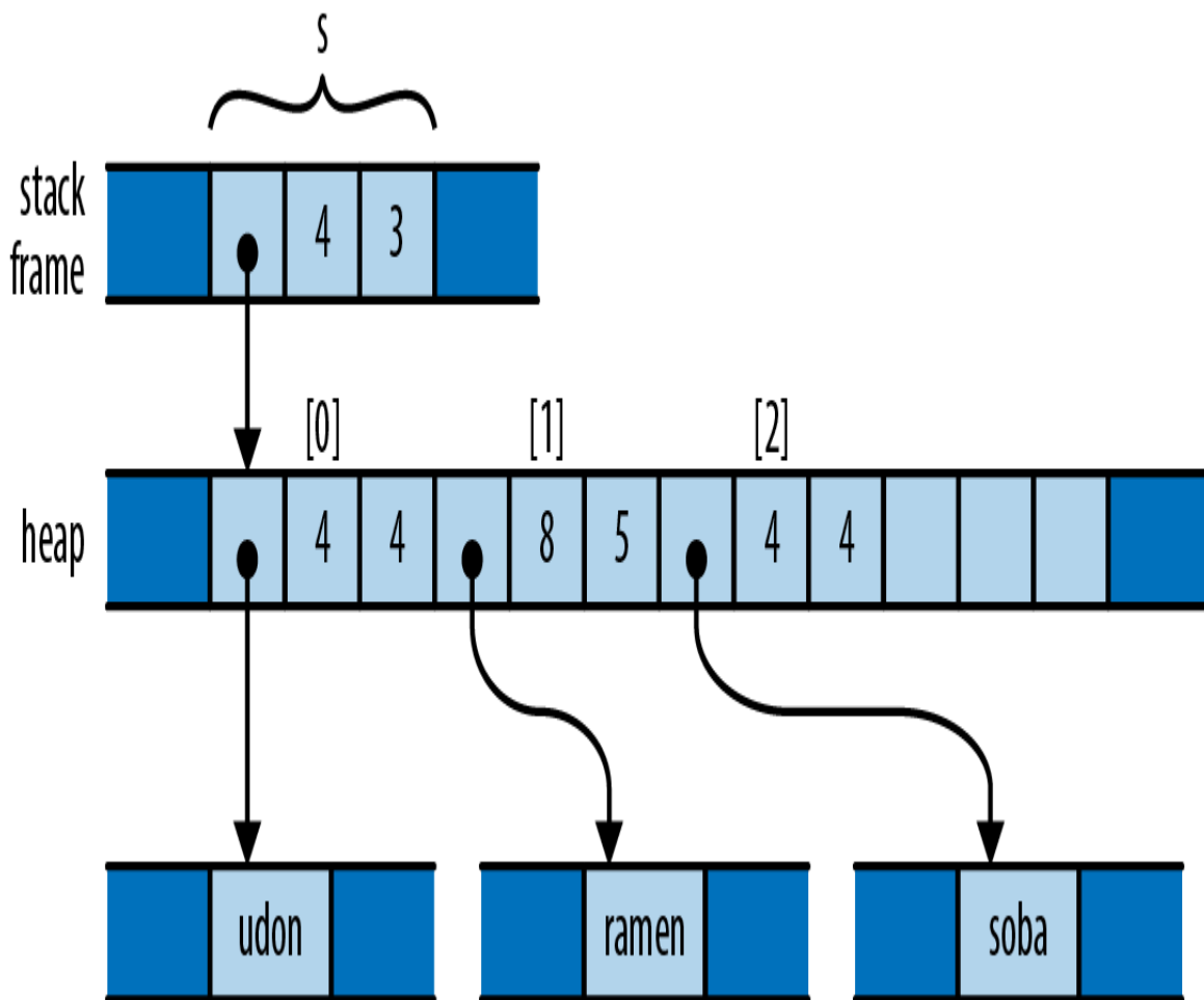
Figure 4-9. How Rust represents a vector of strings in memory
