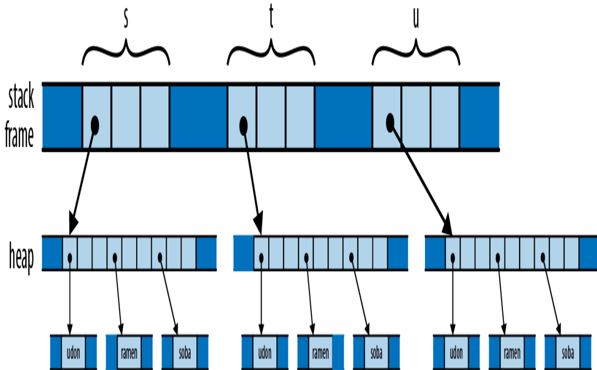
Figure 4-8. The result of assigning s to both t and u in C++
