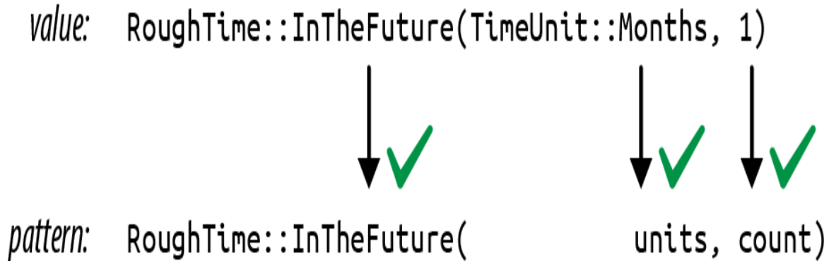
Figure 10-5. A successful match
