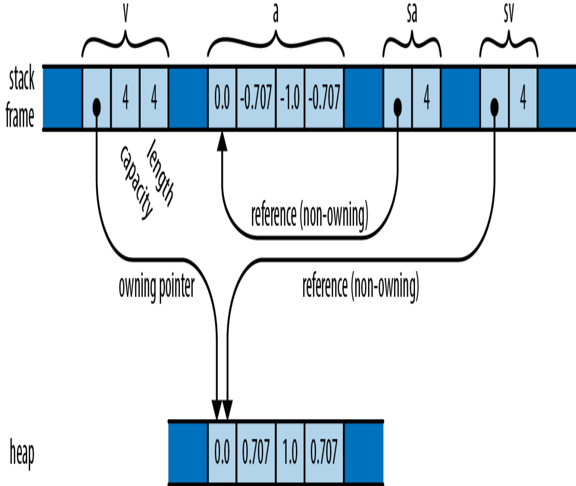
Figure 3-2. A vector v and an array a in memory, with slices sa and sv referring to each
