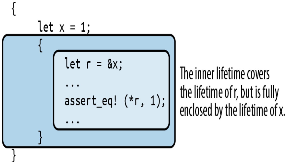
Figure 5-6. A reference with a lifetime enclosing r 's scope, but within x 's scope
