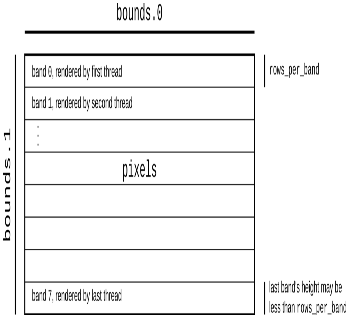
Figure 2-7. Dividing the pixel buffer into bands for parallel rendering
