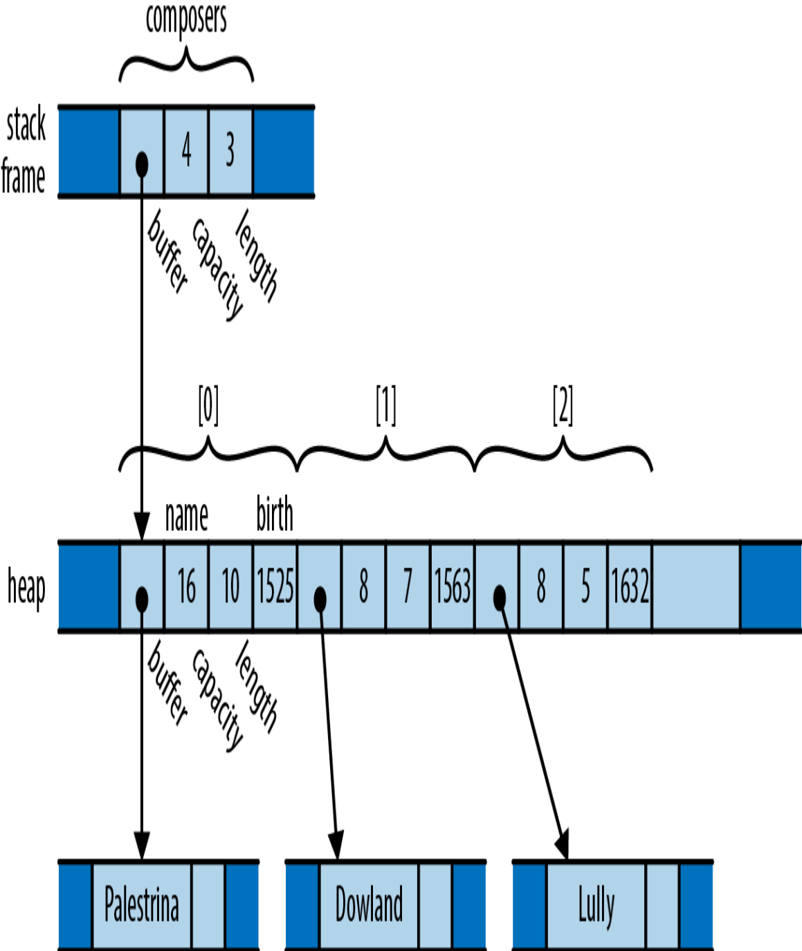
Figure 4-4. A more complex tree of ownership
