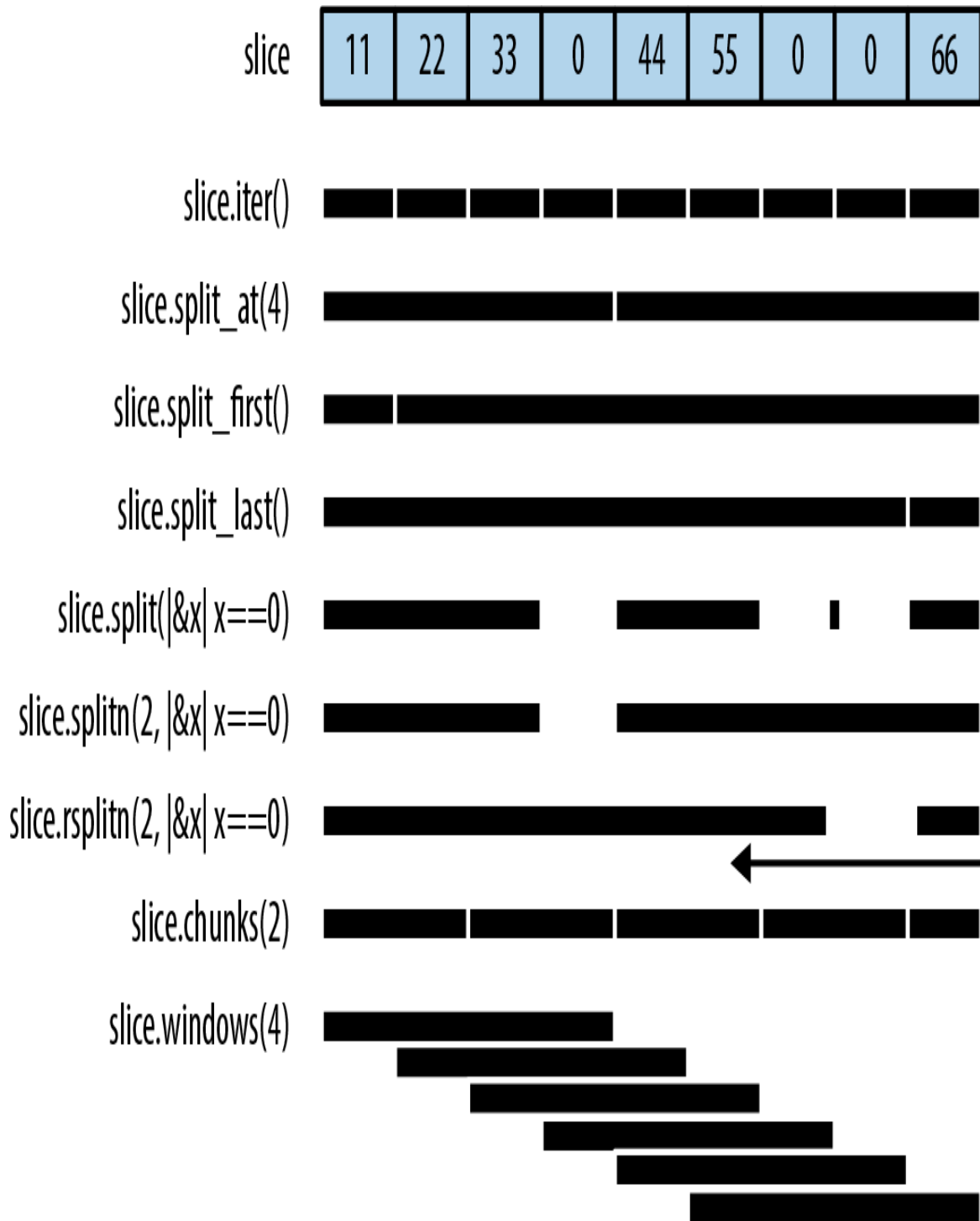
Figure 16-2. Splitting methods illustrated (note: the little rectangle in the output of slice.split() is an empty slice caused by the two adjacent separators, and rsplitn produces its output in end-to-start order, unlike the others)
