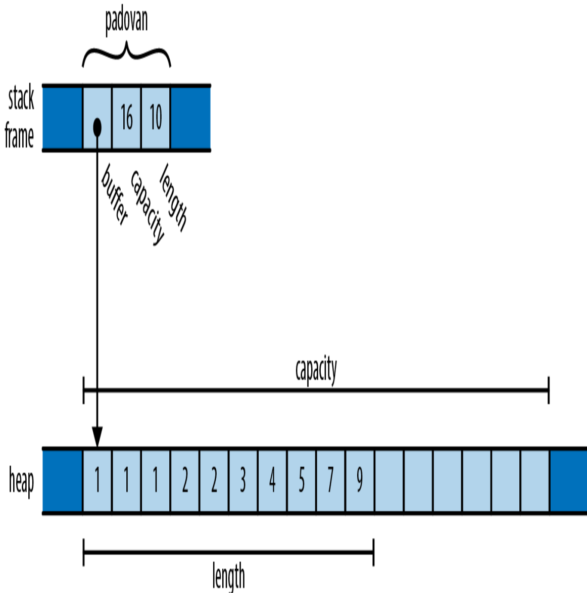
Figure 4-2. A Vec<i32> on the stack, pointing to its buffer in the heap
