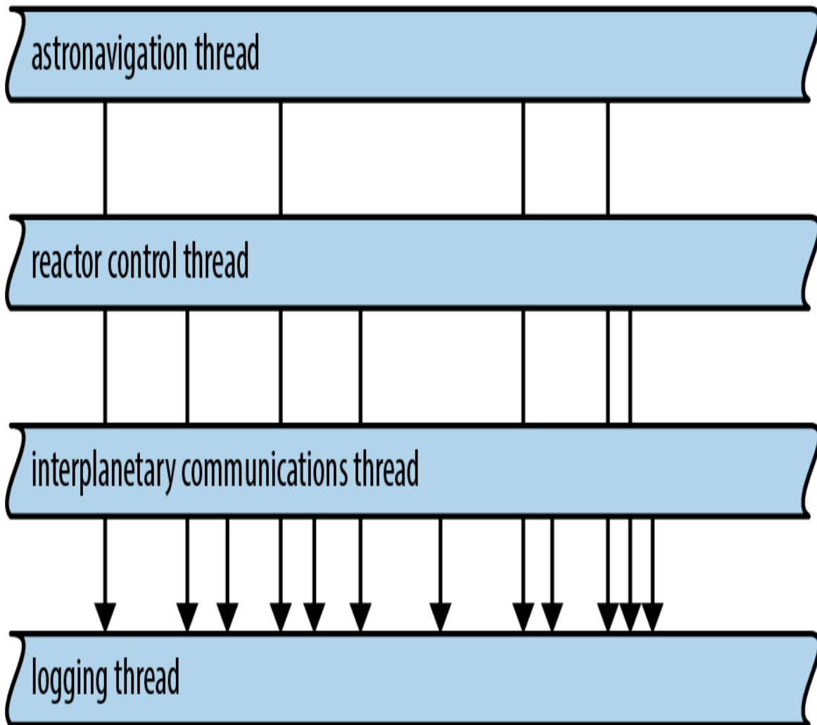
Figure 19-8. A single channel receiving requests from many senders
