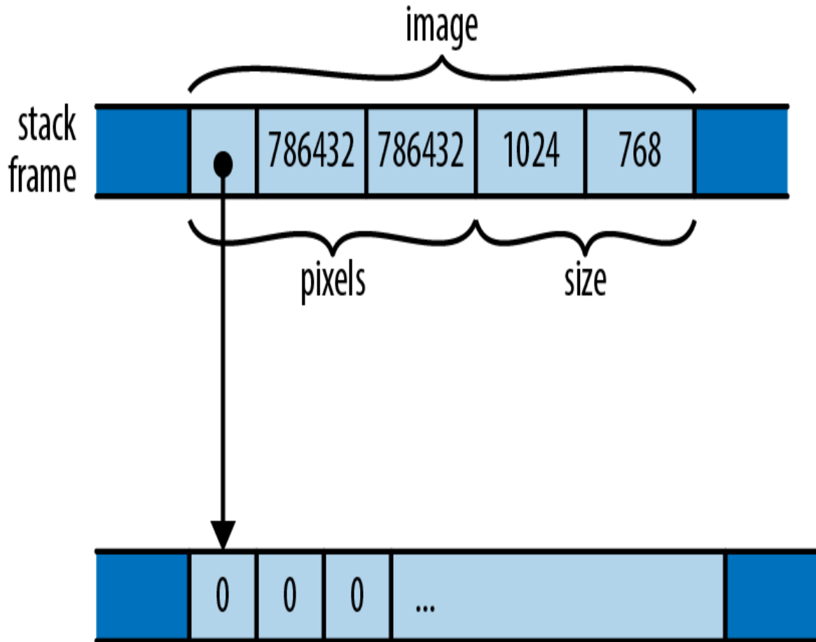
Figure 9-1. A GrayscaleMap structure in memory
