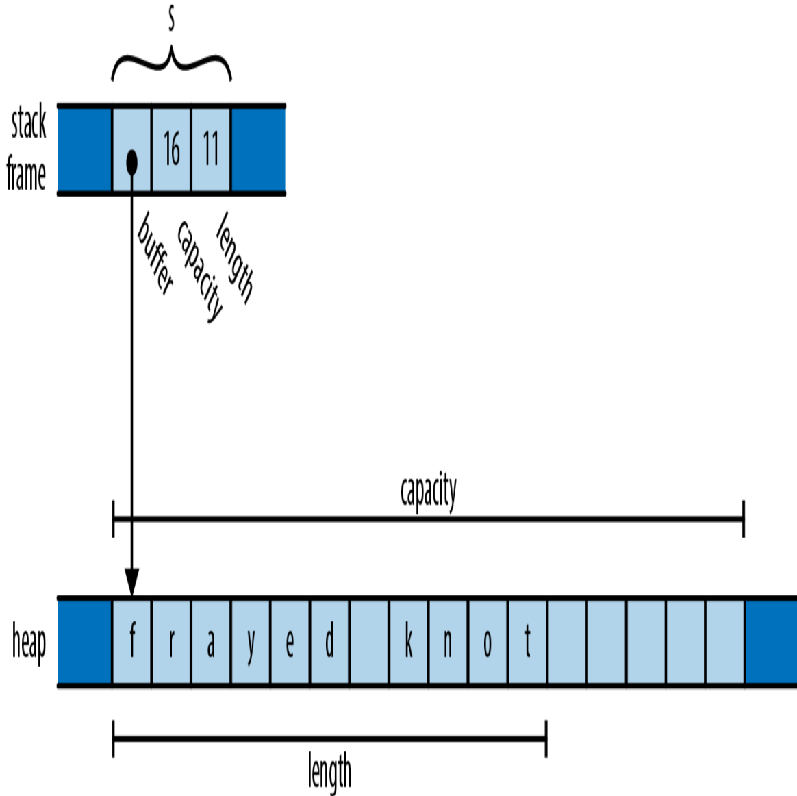
Figure 4-1. A C++ std::string value on the stack, pointing to its heap-allocated buffer
