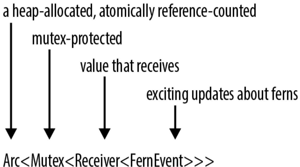
Figure 19-11. How to read a complex type
