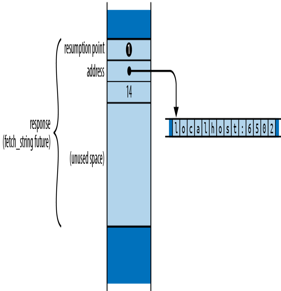
Figure 20-5. The future constructed for a call to fetch_string
