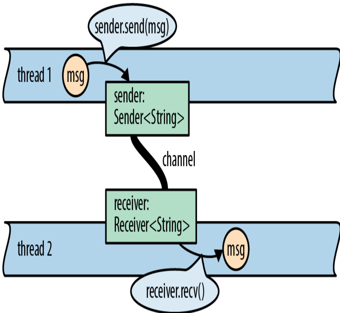
Figure 19-5. A channel for Strings: ownership of the string msg is transferred from thread 1 to thread 2.
