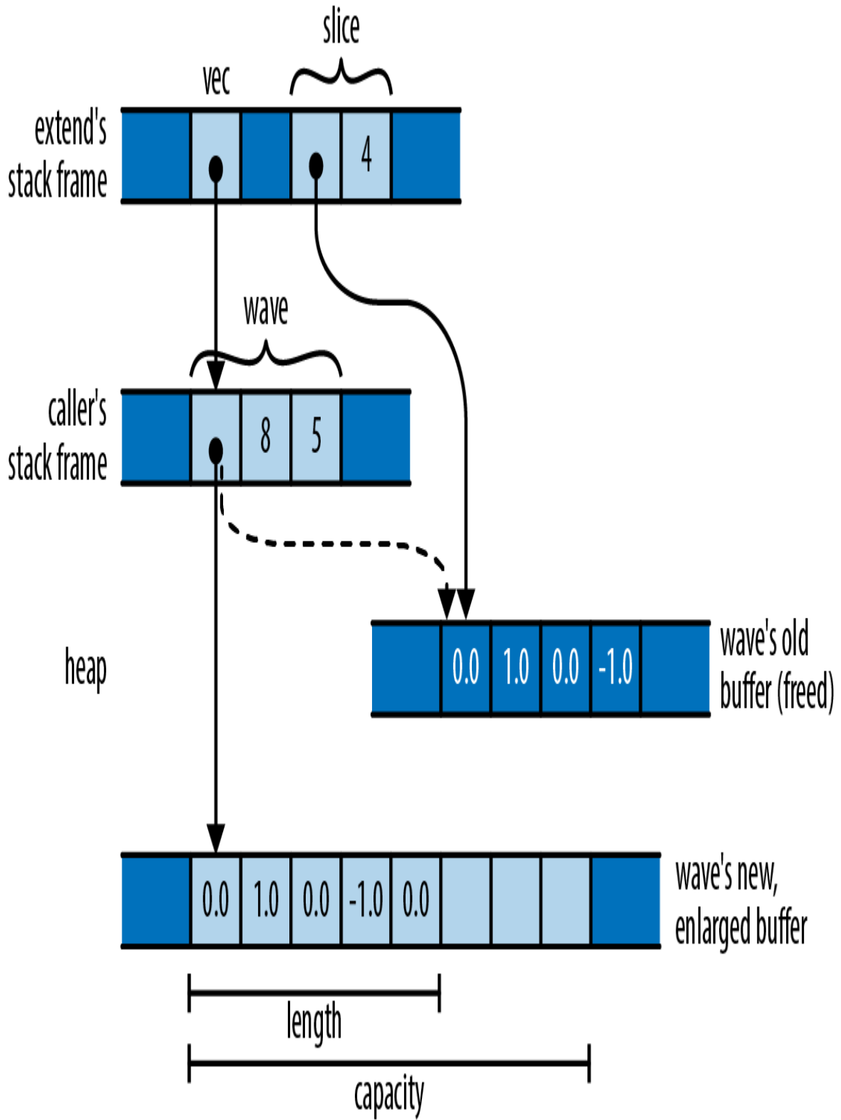
Figure 5-8. A slice turned into a dangling pointer by a vector reallocation
