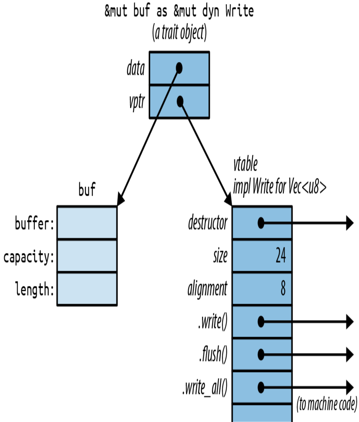
Figure 11-1. Trait objects in memory
