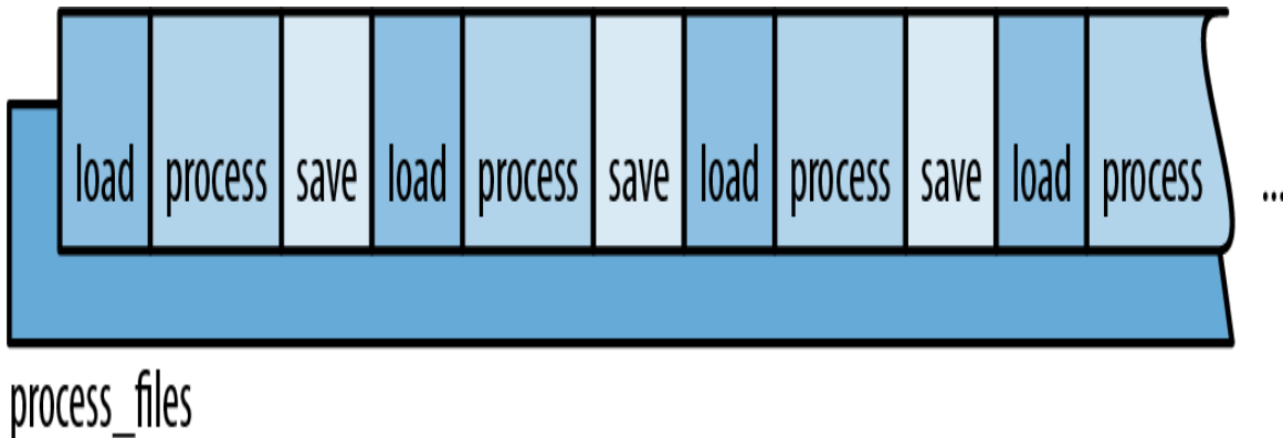
Figure 19-1. Single-threaded execution of process_files()
