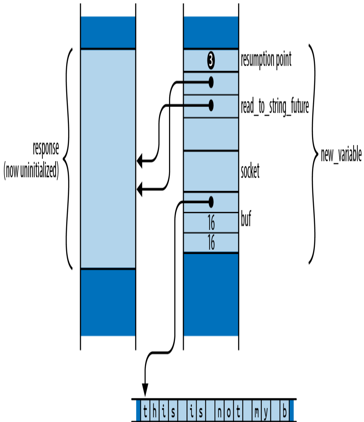
Figure 20-7. fetch_string's future, moved while borrowed (Rust prevents this)
