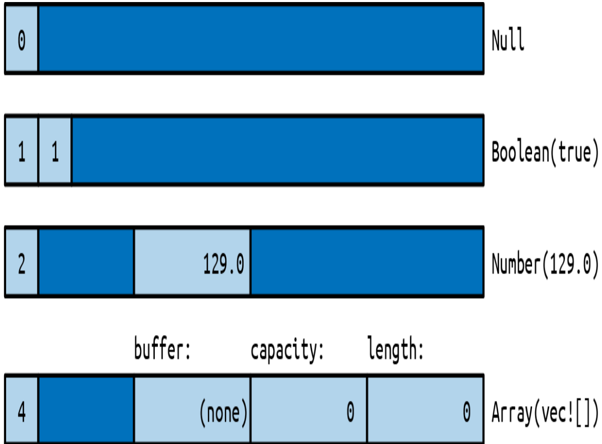
Figure 10-2. Json values in memory
