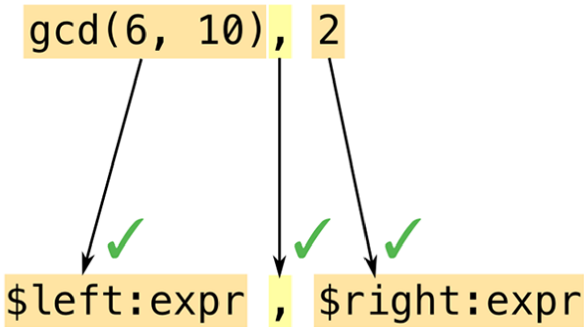
Figure 21-2. Expanding a macro, part 1: pattern-matching the arguments
