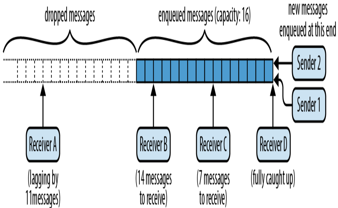
Figure 20-4. A tokio broadcast channel
