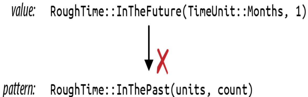
Figure 10-4. A RoughTime value and pattern that do not match
