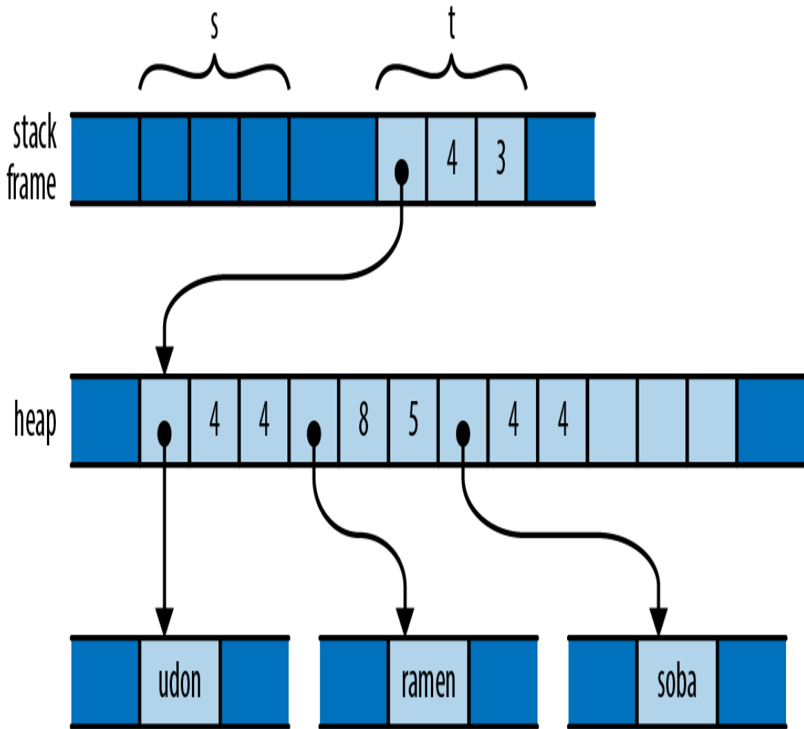
Figure 4-10. The result of assigning s to t in Rust
