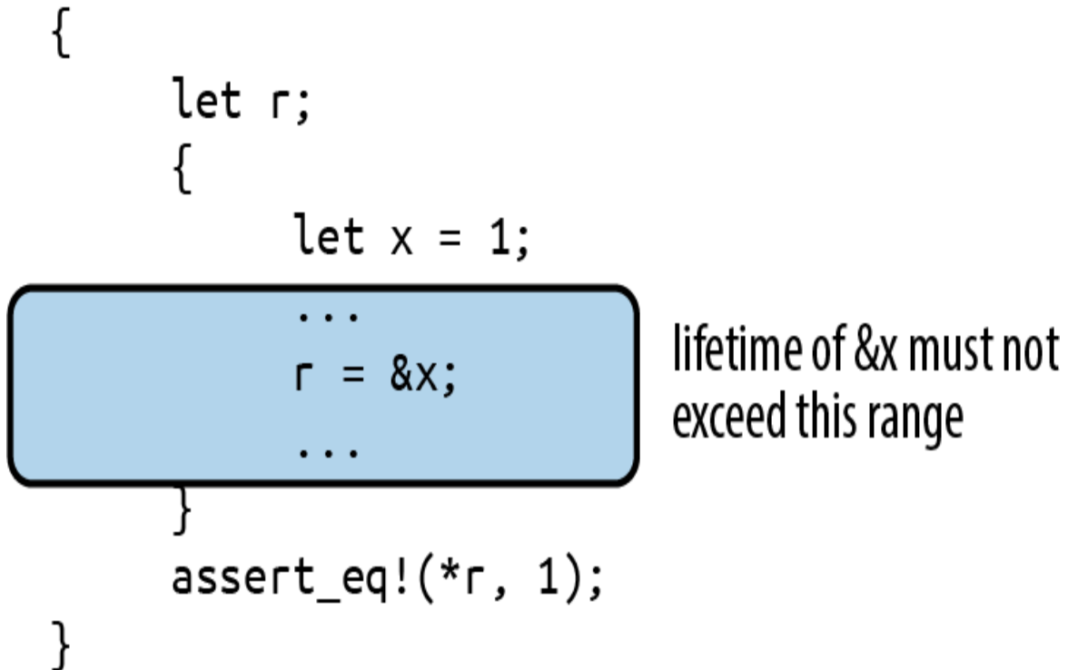
Figure 5-3. Permissible lifetimes for &x
