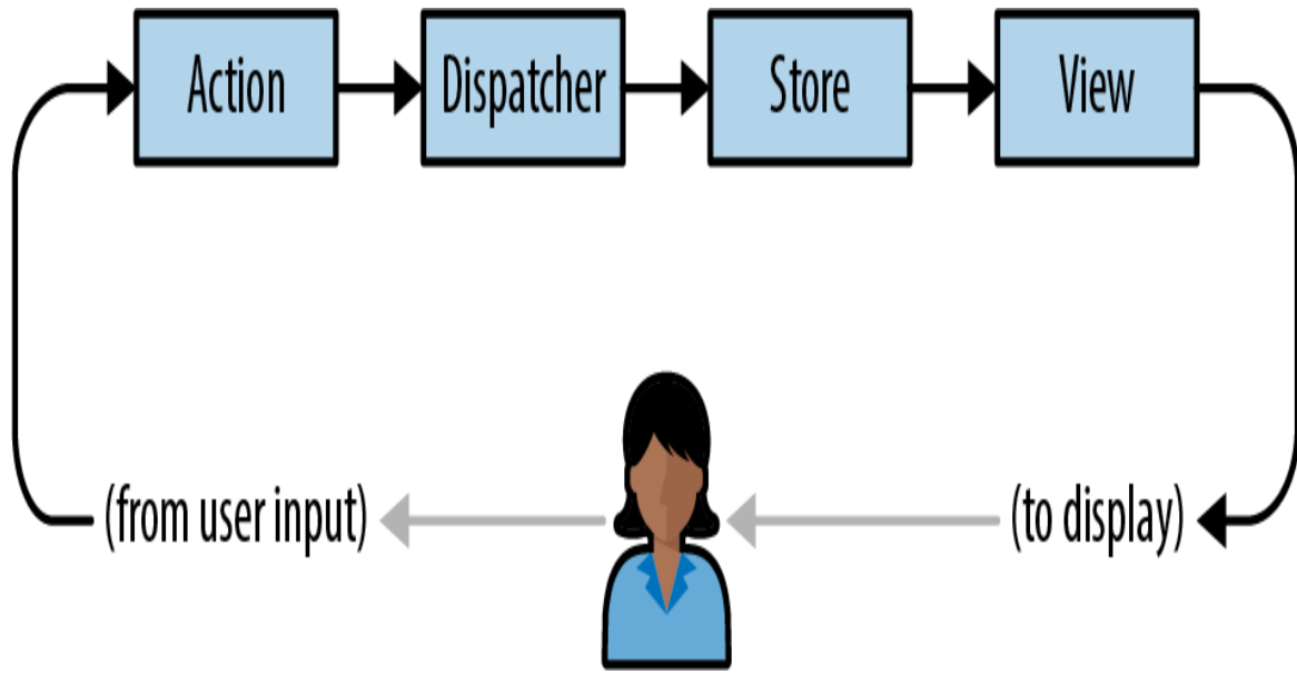
Figure 14-4. The Flux architecture, an alternative to MVC
