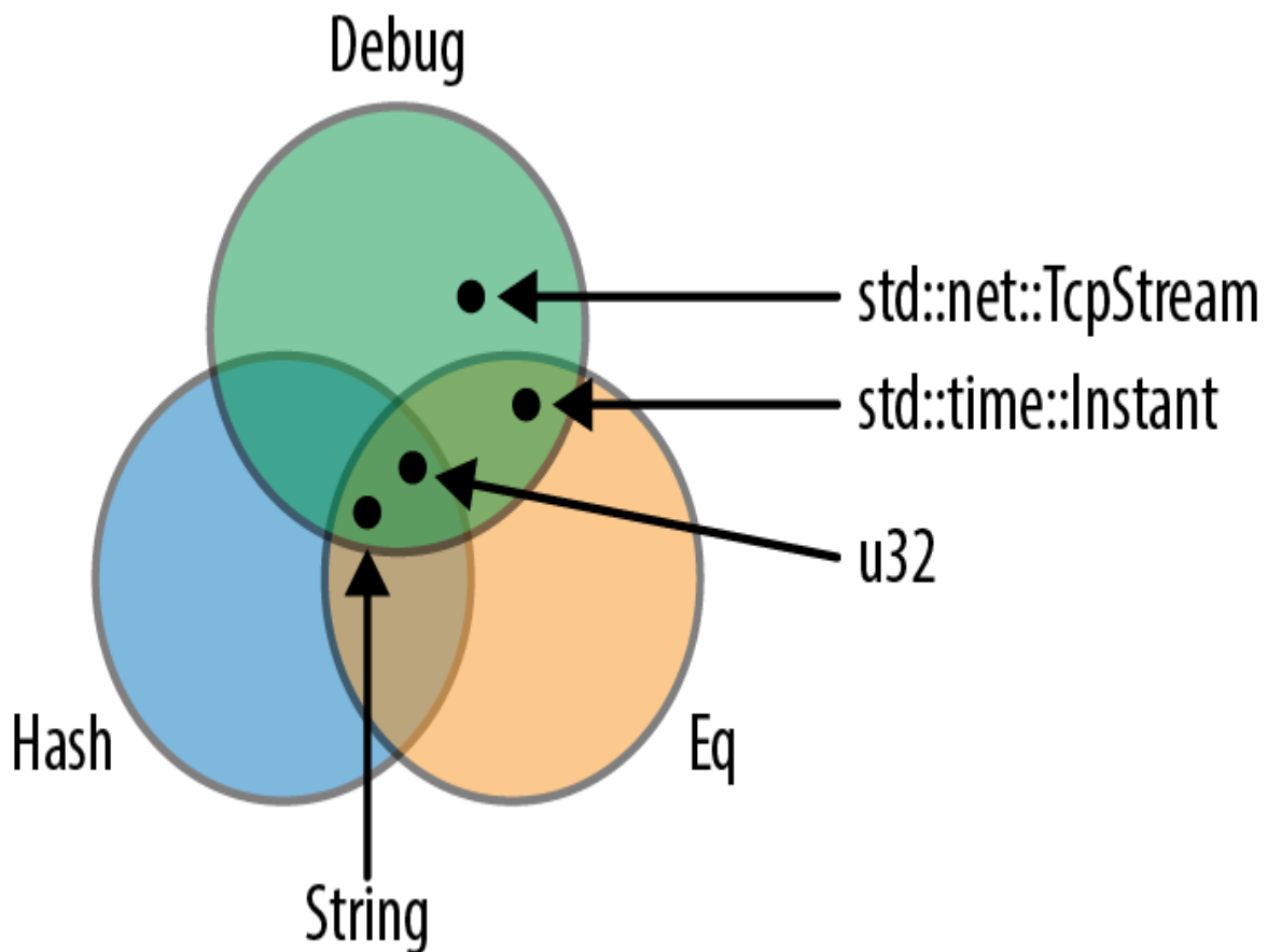
Figure 11-2. Traits as sets of types
