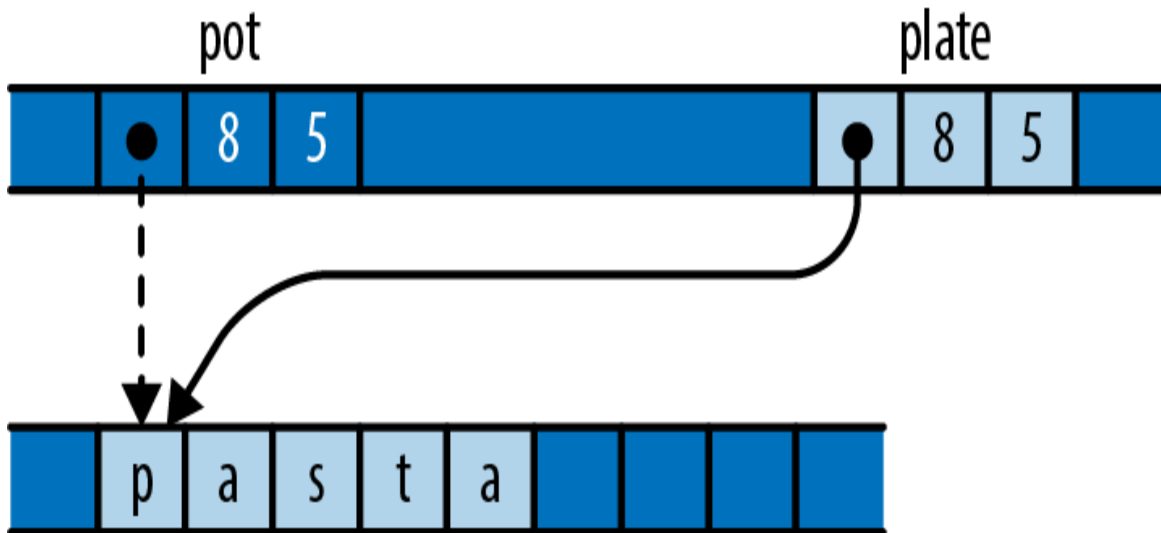
Figure 22-2. Moving a string from one local variable to another
