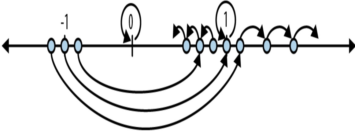
Figure 2-3. Effects of repeatedly squaring a number
