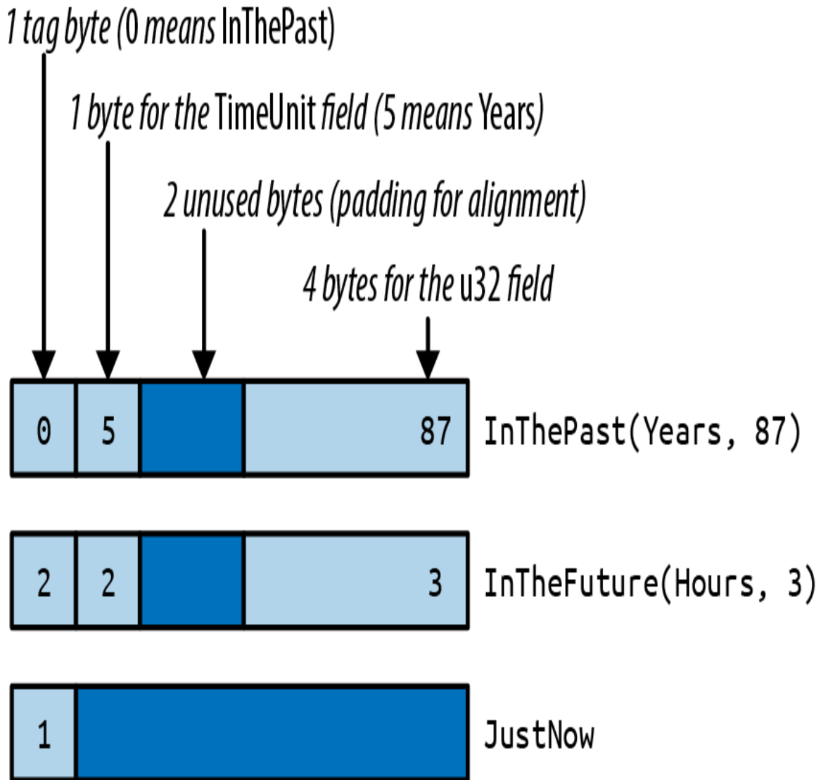
Figure 10-1. RoughTime values in memory
