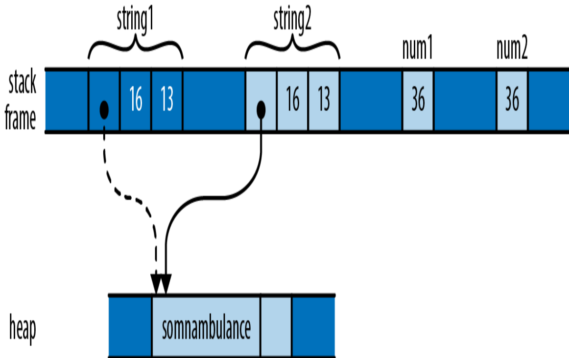
Figure 4-11. Assigning a String moves the value, whereas assigning an i32 copies it
