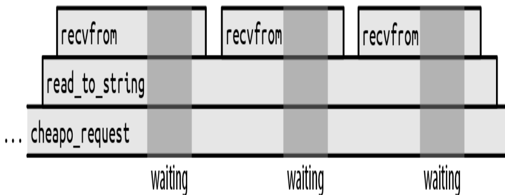
Figure 20-1. Progress of a synchronous HTTP request (darker gray areas are waiting for the operating system)
