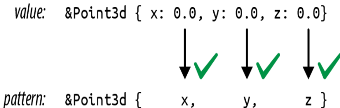
Figure 10-7. Pattern matching with references
