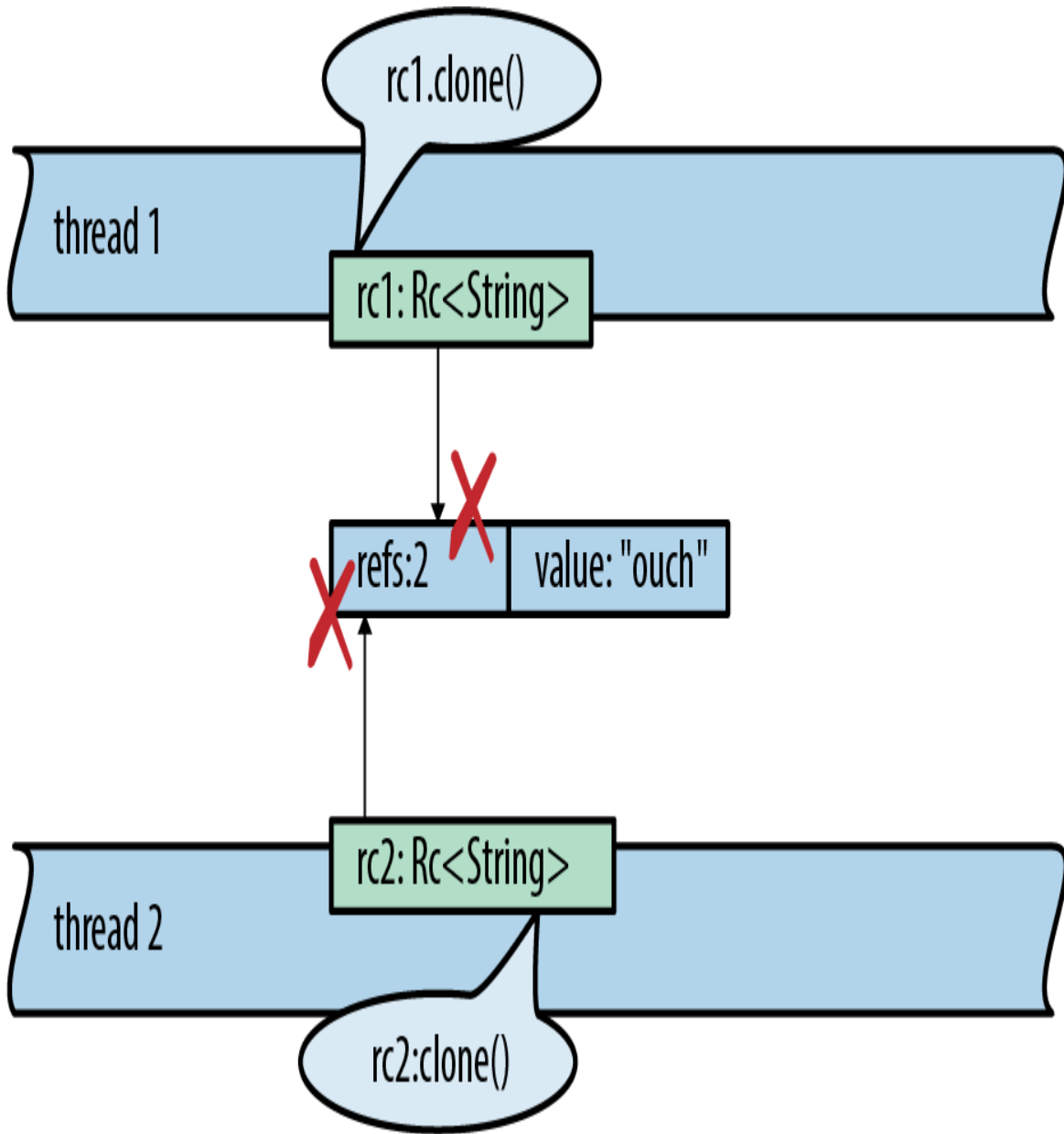
Figure 19-10. Why Rc<String> is neither Sync nor Send
