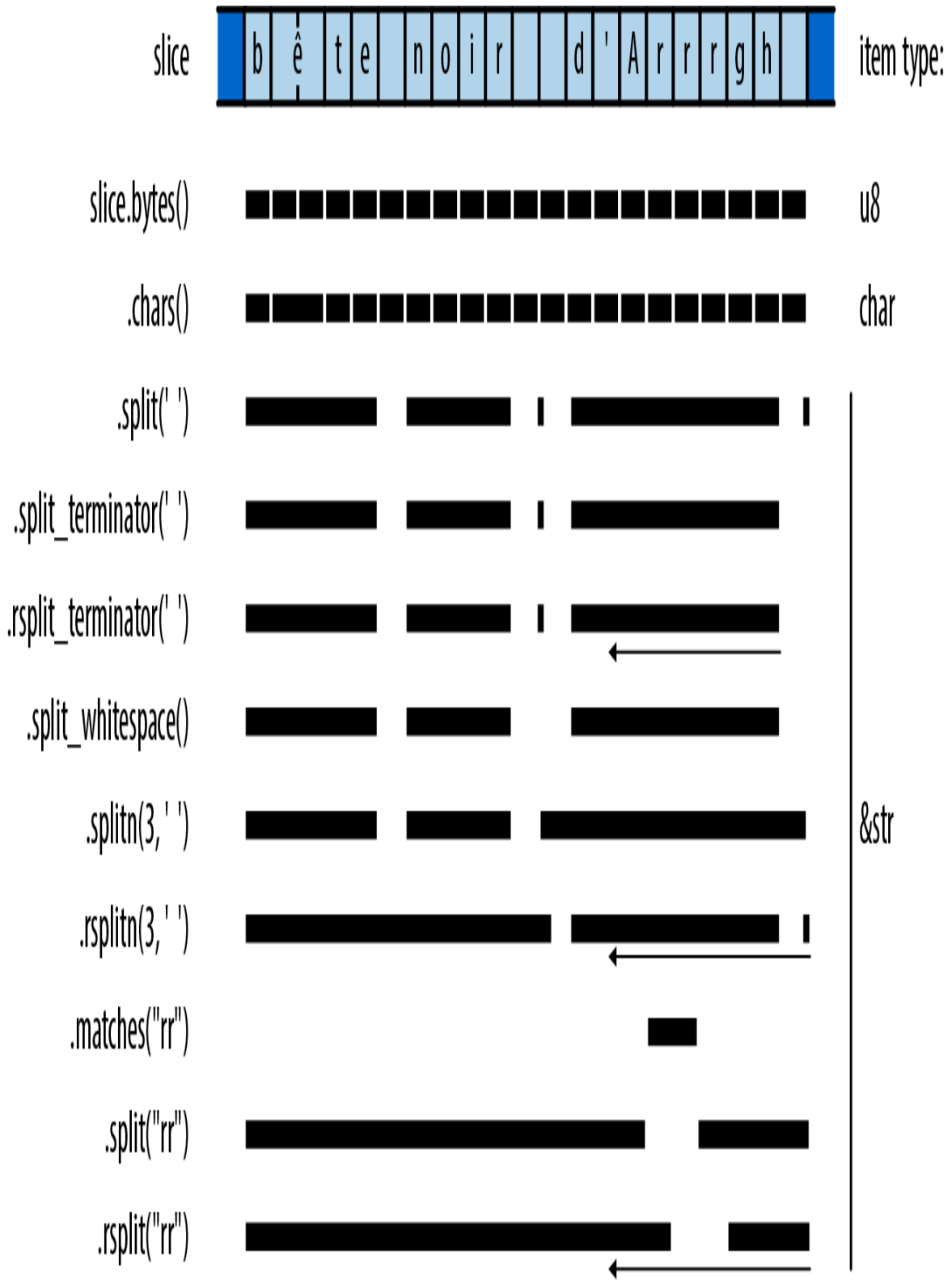
Figure 17-3. Some ways to iterate over a slice
