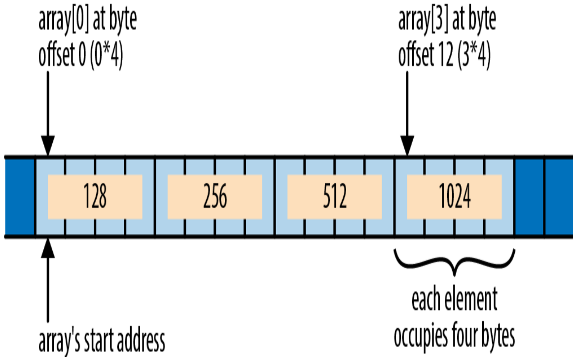
Figure 22-1. An array in memory
