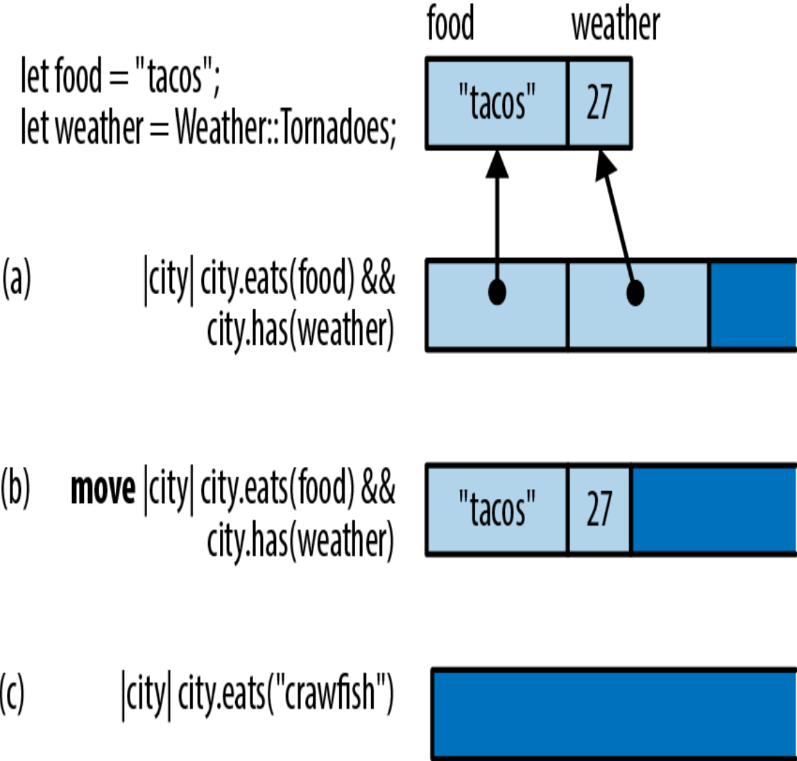
Figure 14-1. Layout of closures in memory
