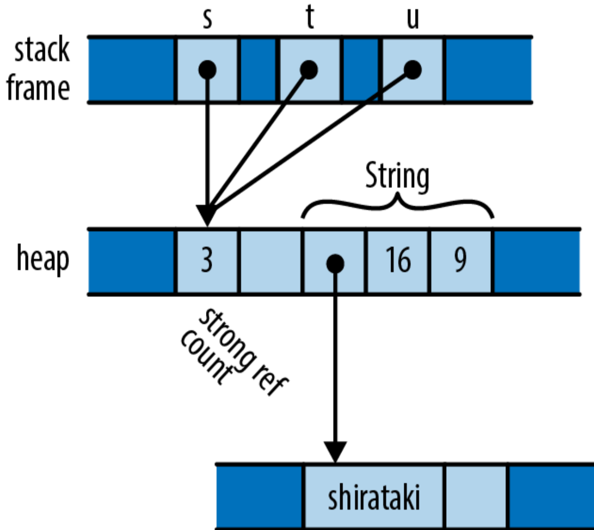
Figure 4-12. A reference-counted string with three references
