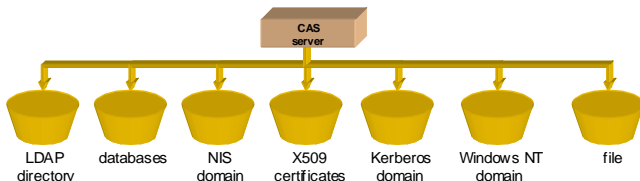
Figure 12: User authentication with ESUP-Portail GenericHandler
