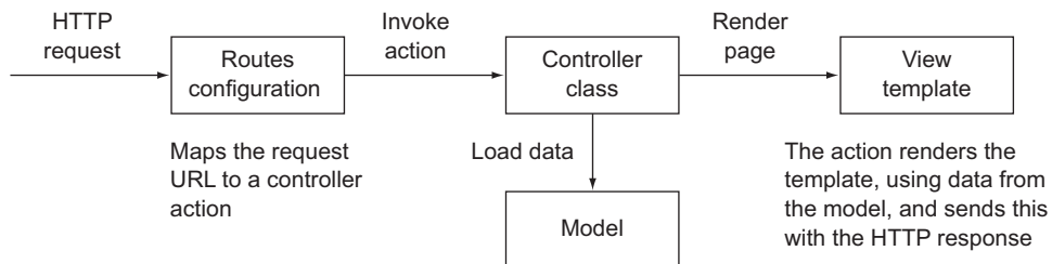
Figure 2.2 The application's model-view-controller structure
