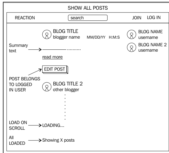
Post list view
