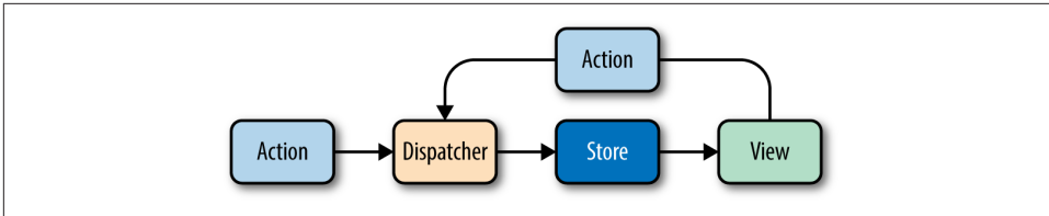
Figure 9-12. Data propagation in the Flux architecture
