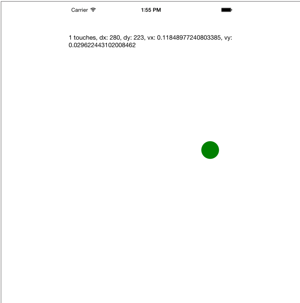
Figure 4-4. PanResponder demo
