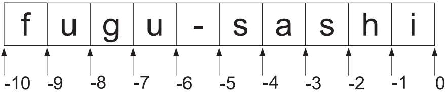
Figure 1-2. Negative indexing
