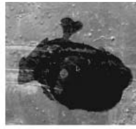
Subtractive blending
