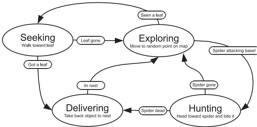
Figure 7-3. Ant state machine
