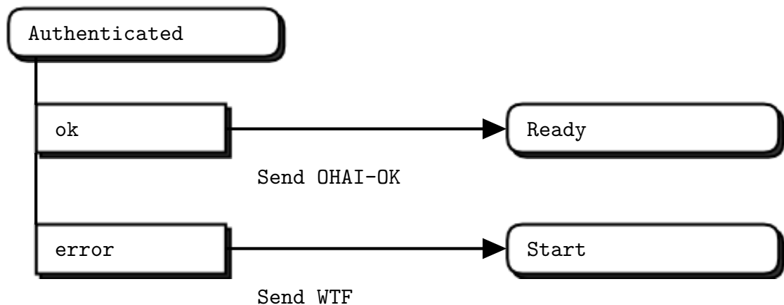
Figure 7-2. The Authenticated State
