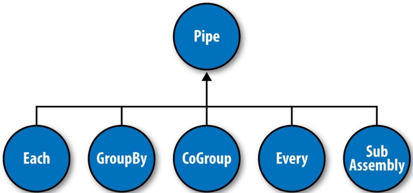
Figure 24-3. Pipe types
