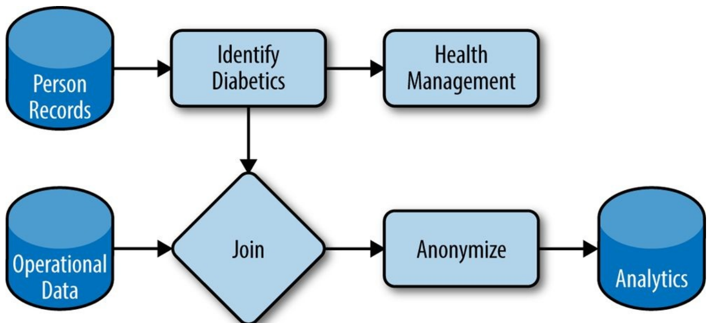
Figure 22-2. Composable datasets and functions
