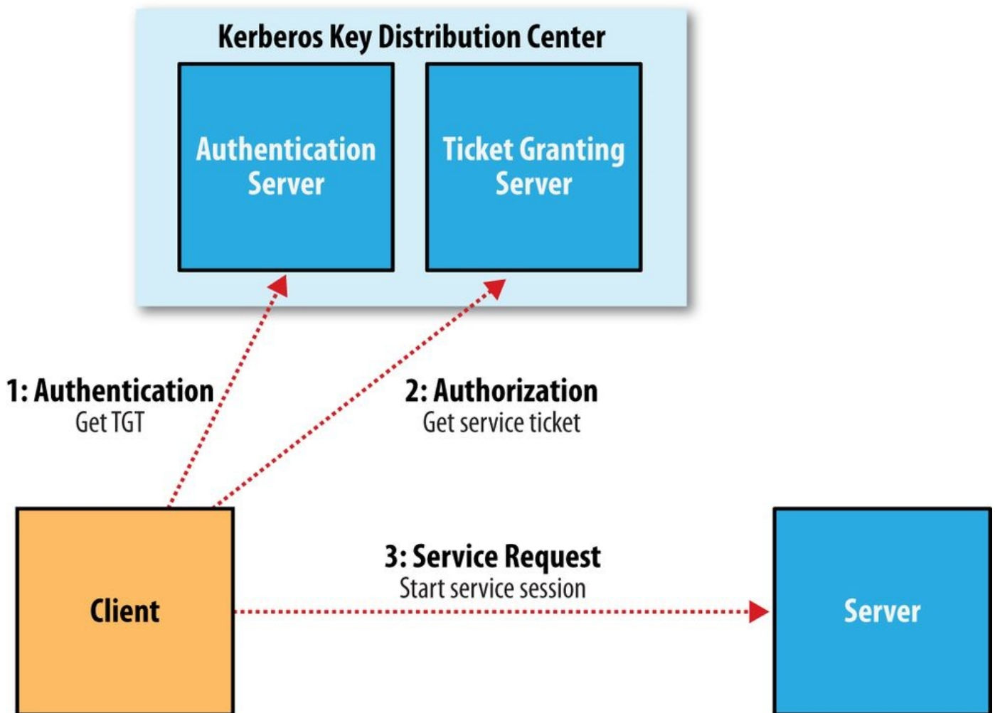
Figure 10-2. The three-step Kerberos ticket exchange protocol
