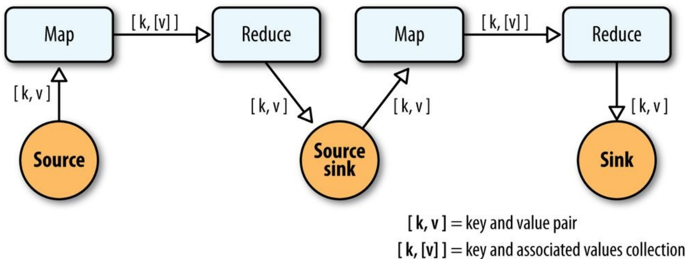
Figure 24-1. Counting and sorting in MapReduce
