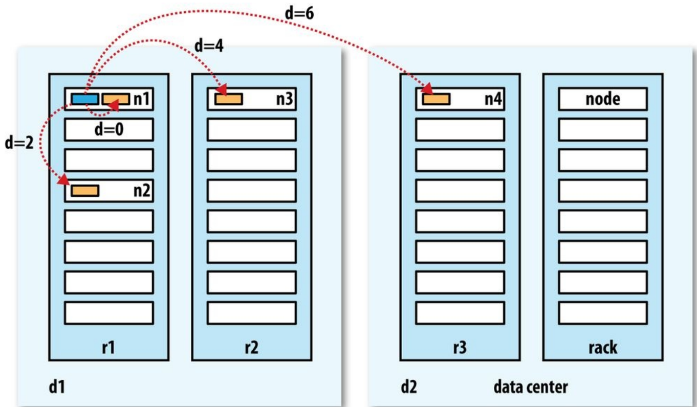
Figure 3-3. Network distance in Hadoop
