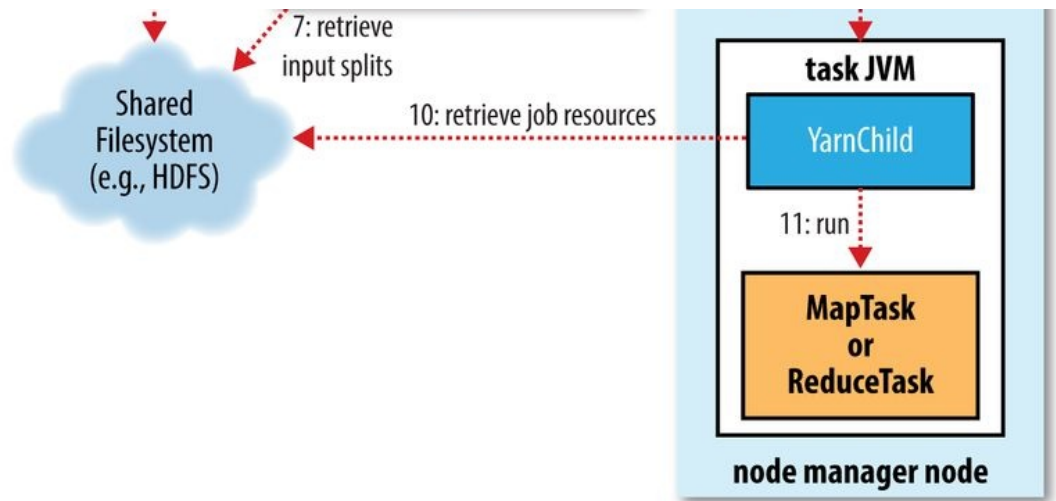
Figure 7-1. How Hadoop runs a MapReduce job
