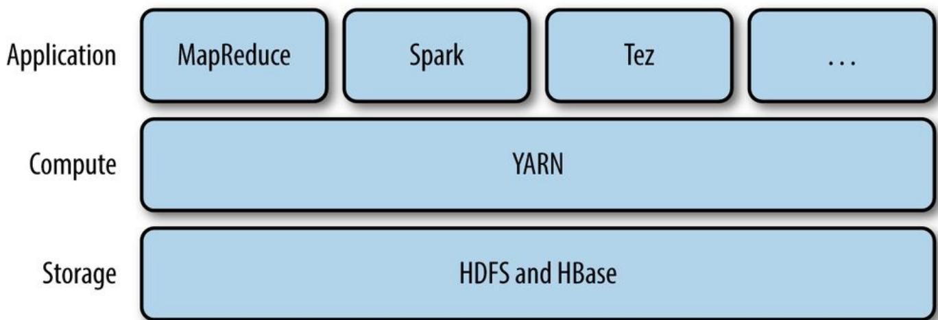
Figure 4-1. YARN applications
