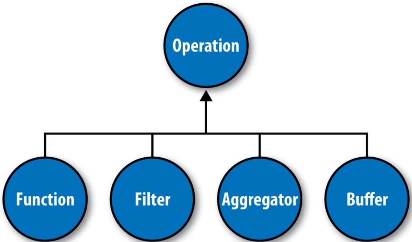
Figure 24-5. Operation types
