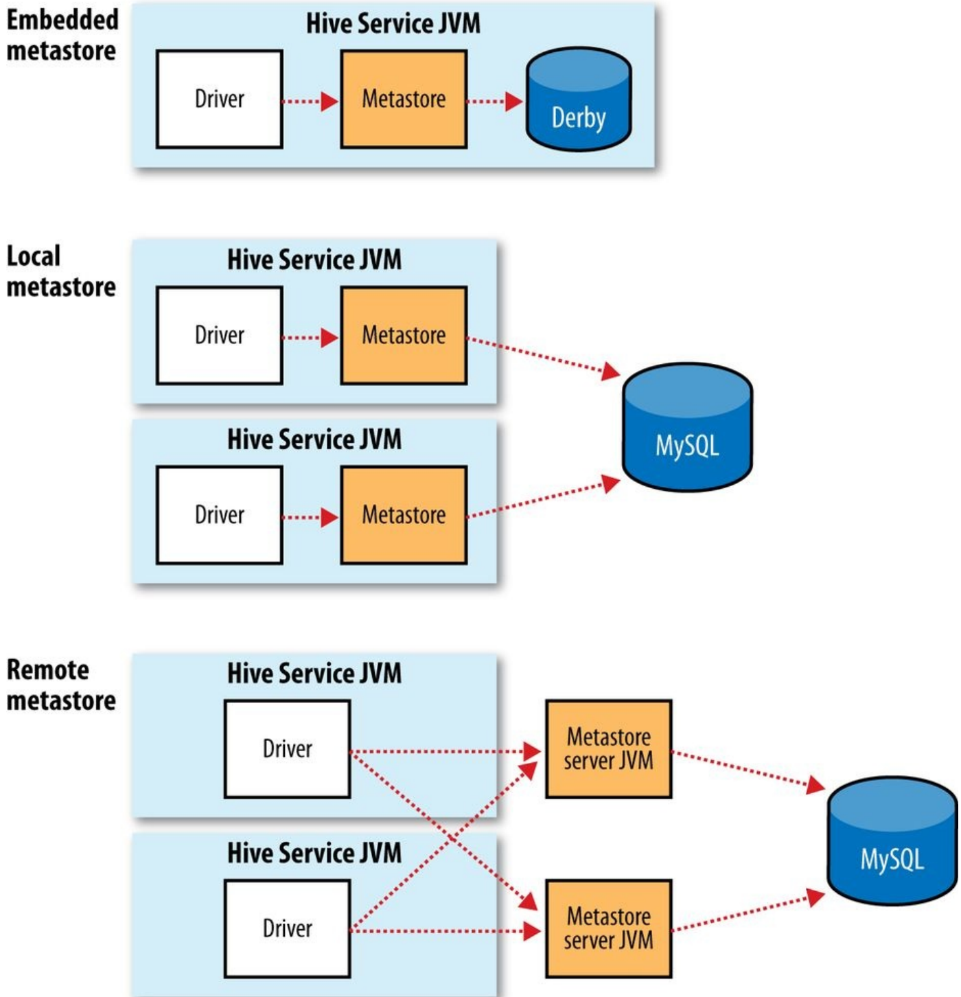
Figure 17-2. Metastore configurations
