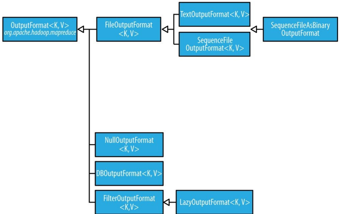
Figure 8-4. OutputFormat class hierarchy
