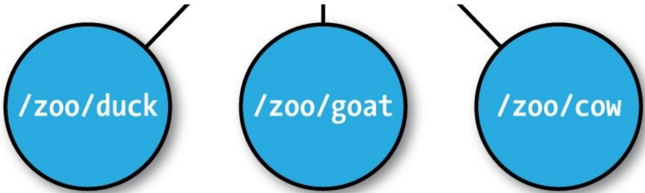
Figure 21-1. ZooKeeper znodes
