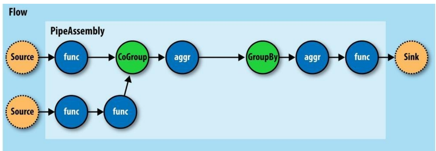
Figure 24-7. A Flow
