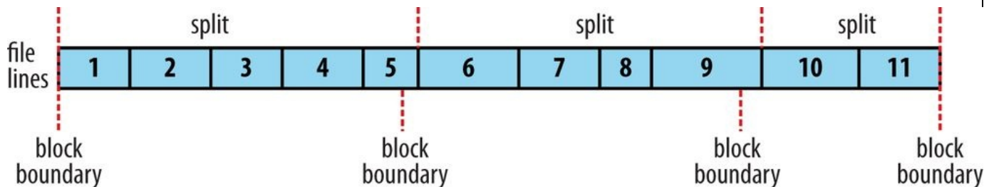
Figure 8-3. Logical records and HDFS blocks for TextInputFormat
