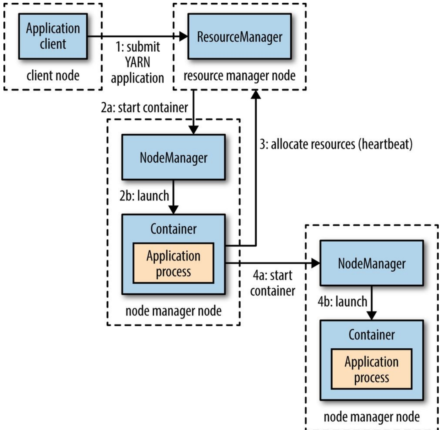
Figure 4-2. How YARN runs an application
