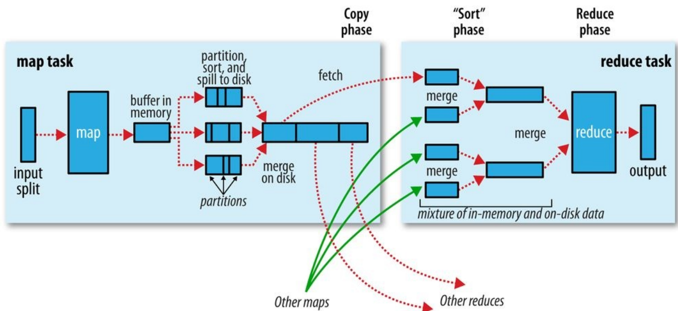
Figure 7-4. Shuffle and sort in MapReduce
