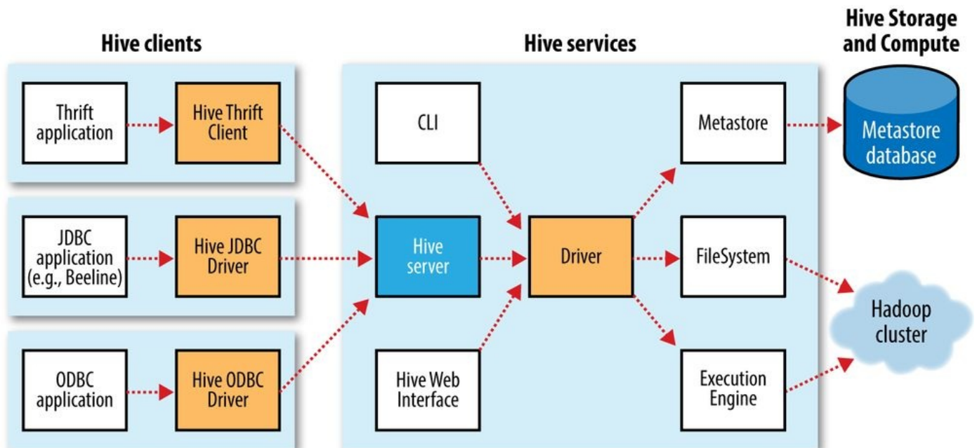
Figure 17-1. Hive architecture
