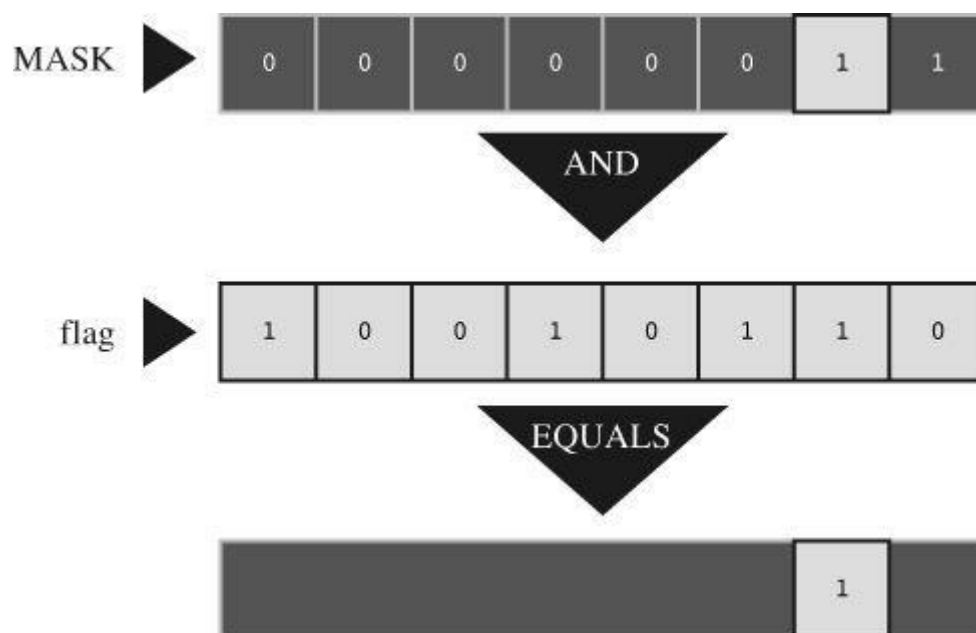
Figure 15.2 A mask.
