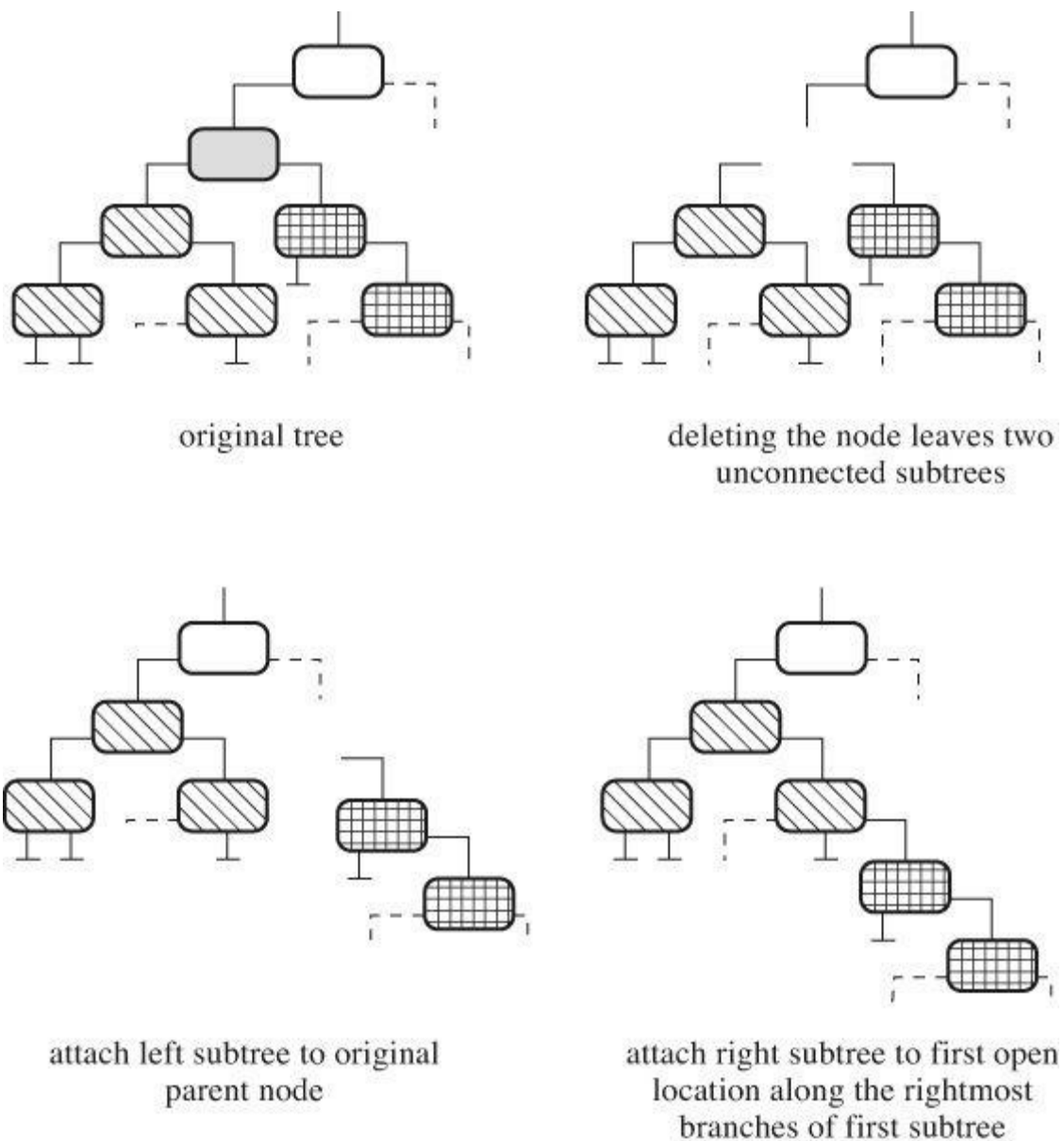
Figure 17.15 Deleting a two-child node.
