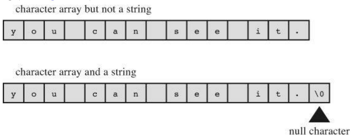
Figure 6.6 Character arrays and strings.
