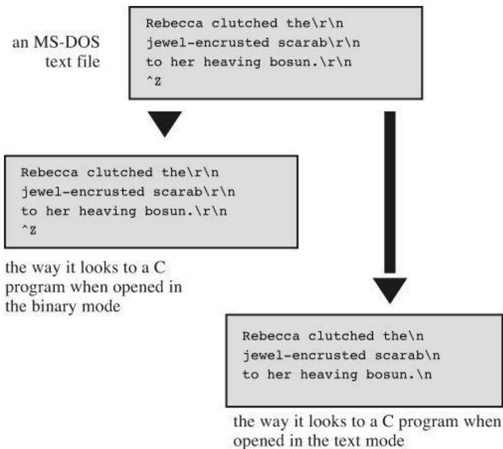
Figure 13.1 Binary view and text view.
