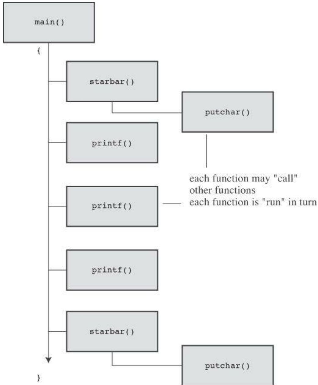
Figure 9.1 Control flow for 1ethead1.c ( Listing 9.1 ).
