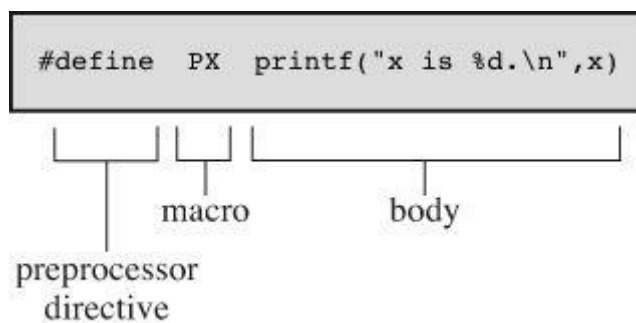
Figure 16.1 Parts of an object-like macro definition.
