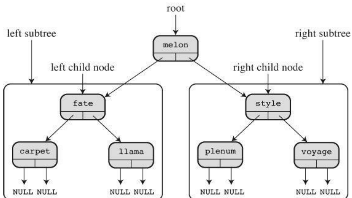
Figure 17.12 A binary search tree storing words.
