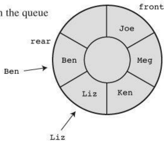
Circular queue wraps around to front of array
