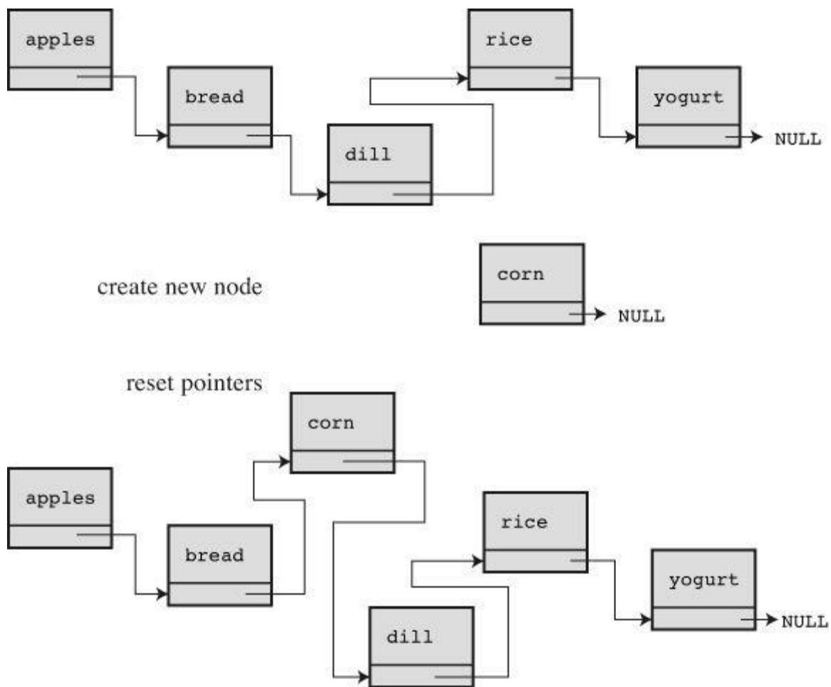
Figure 17.10 Inserting an element into a linked list.
