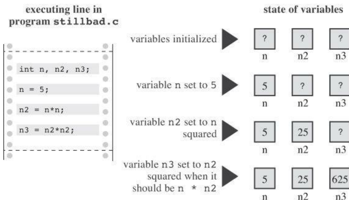
Figure 2.6 Tracing a program.
