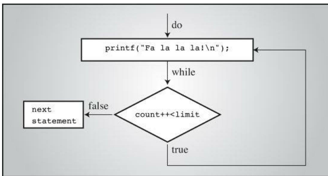
Figure 6.5 Structure of a do while loop.
