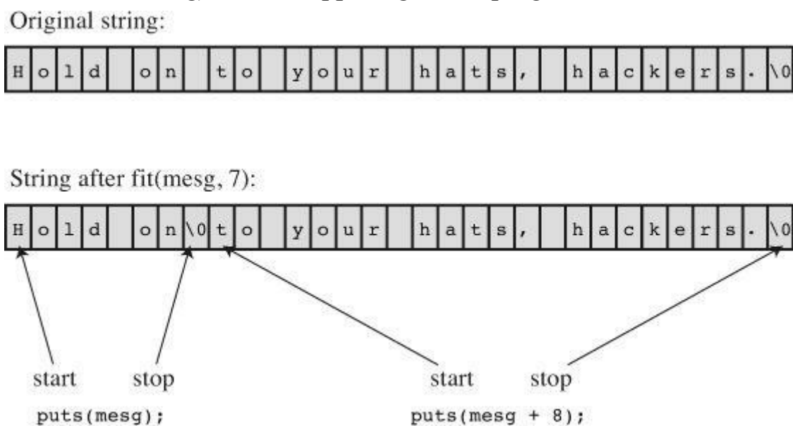
Figure 11.4 The puts() function and the null character.
