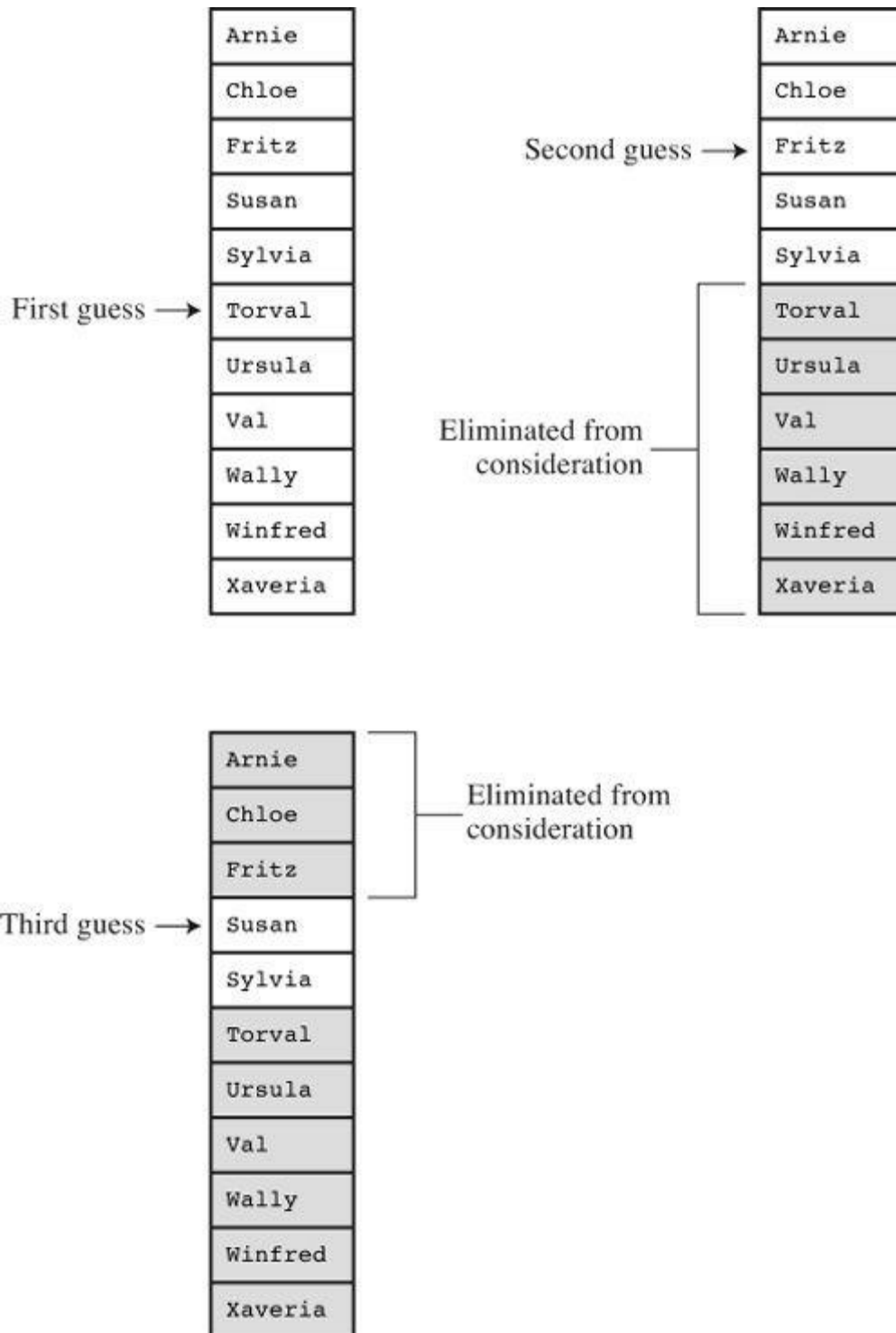
Figure 17.11 A binary search for Susan.
