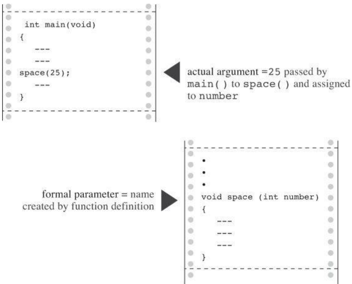
Figure 9.3 Formal parameters and actual arguments.
