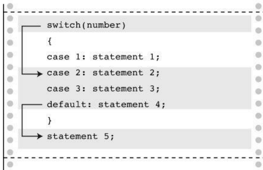
Figure 7.4 Program flow in switches, with and without breaks.
