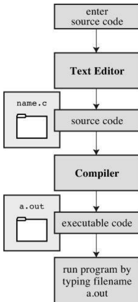
Figure 1.5 Preparing a C program using Unix.
