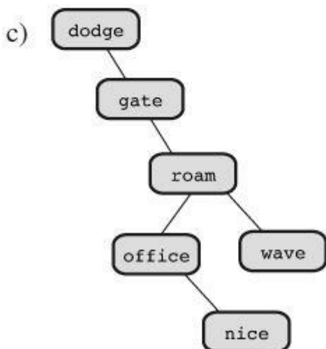
Figure A.2 Binary search tree of words after removal.
