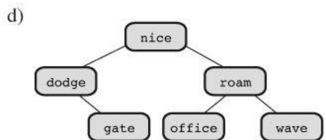
Figure A.2 Binary search tree of words after removal.
