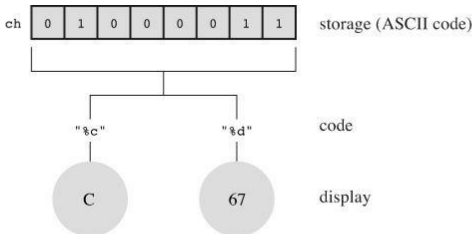
Figure 3.6 Data display versus data storage.
