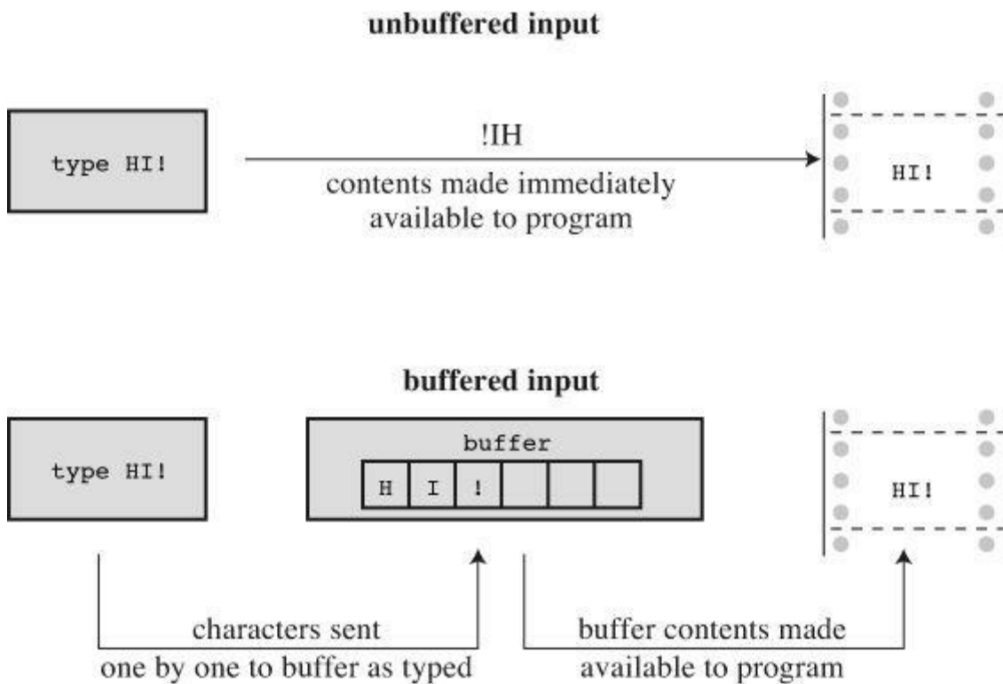
Figure 8.1 Buffered versus unbuffered input.
