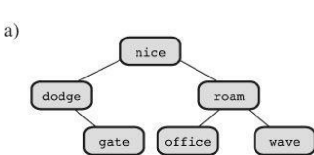
Figure A.1 Binary search tree of words.
