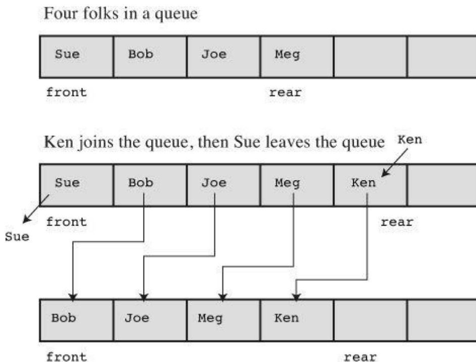
Figure 17.6 Using an array as a queue.
