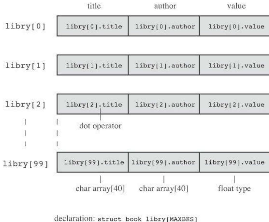
Figure 14.2 An array of structures.
