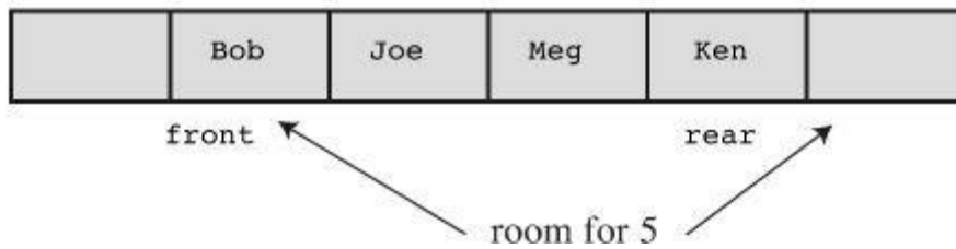
Figure 17.7 Redefining the front element.
