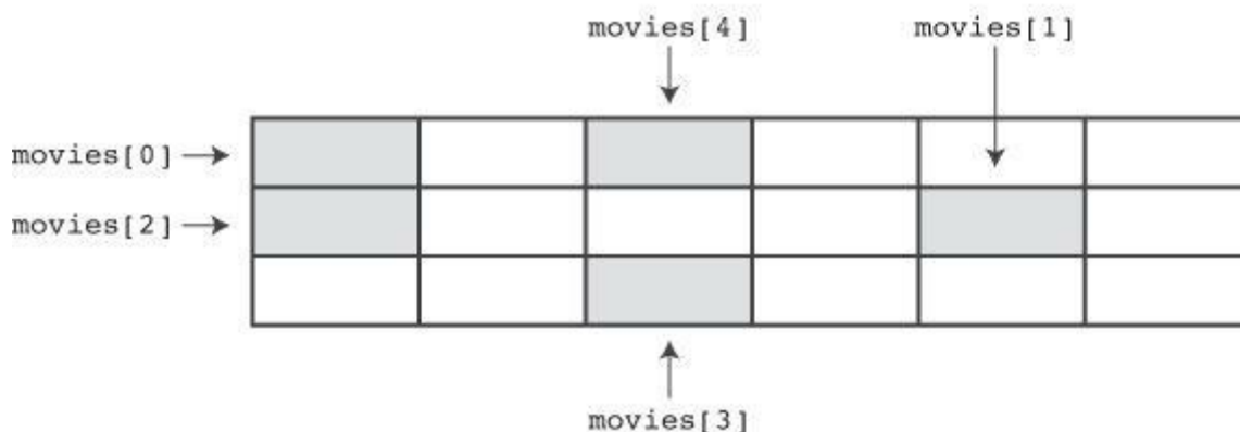
Figure 17.1 Allocating structures in a block versus allocating them individually.
