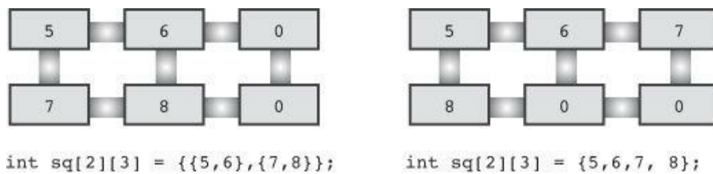
Figure 10.2 Two methods of initializing an array.
