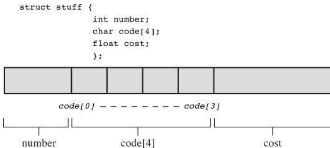
Figure 14.1 Memory allocation for a structure.
