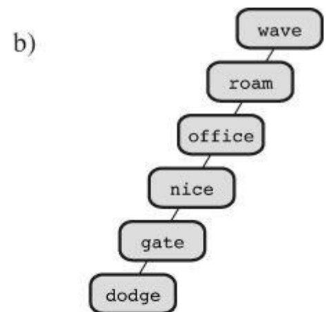
Figure A.1 Binary search tree of words.
