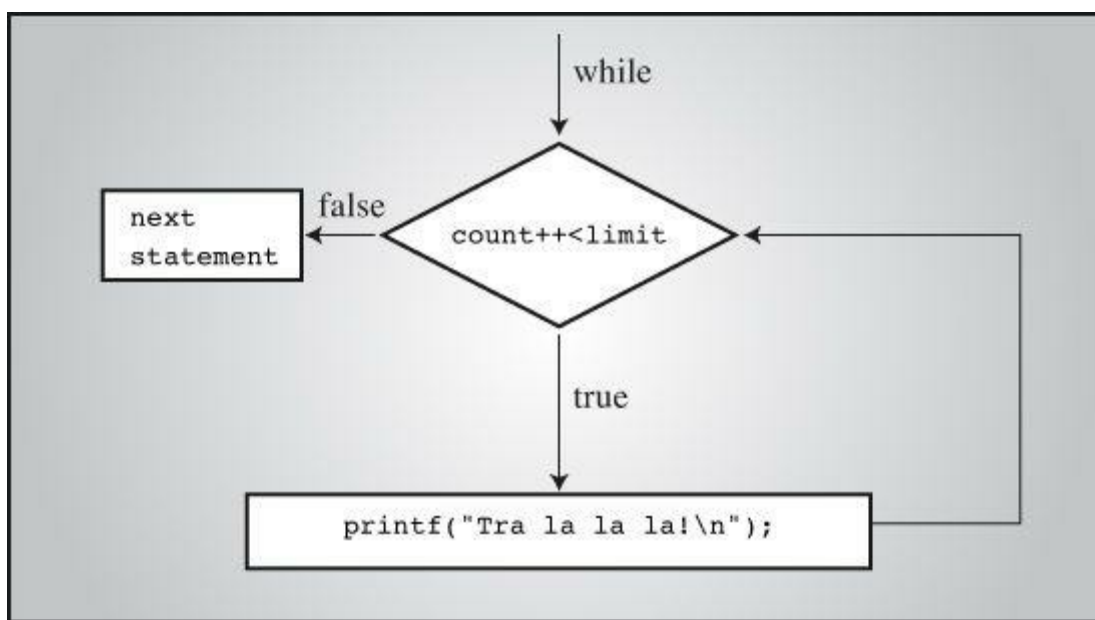
Figure 6.1 Structure of the while loop.
