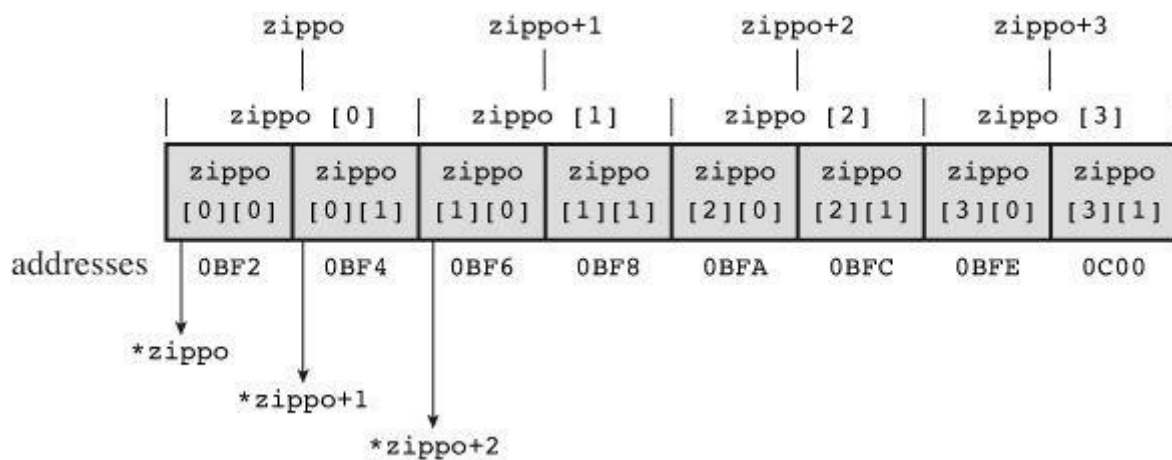
Figure 10.5 An array of arrays.
