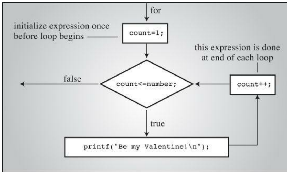
Figure 6.3 Structure of a for loop.
