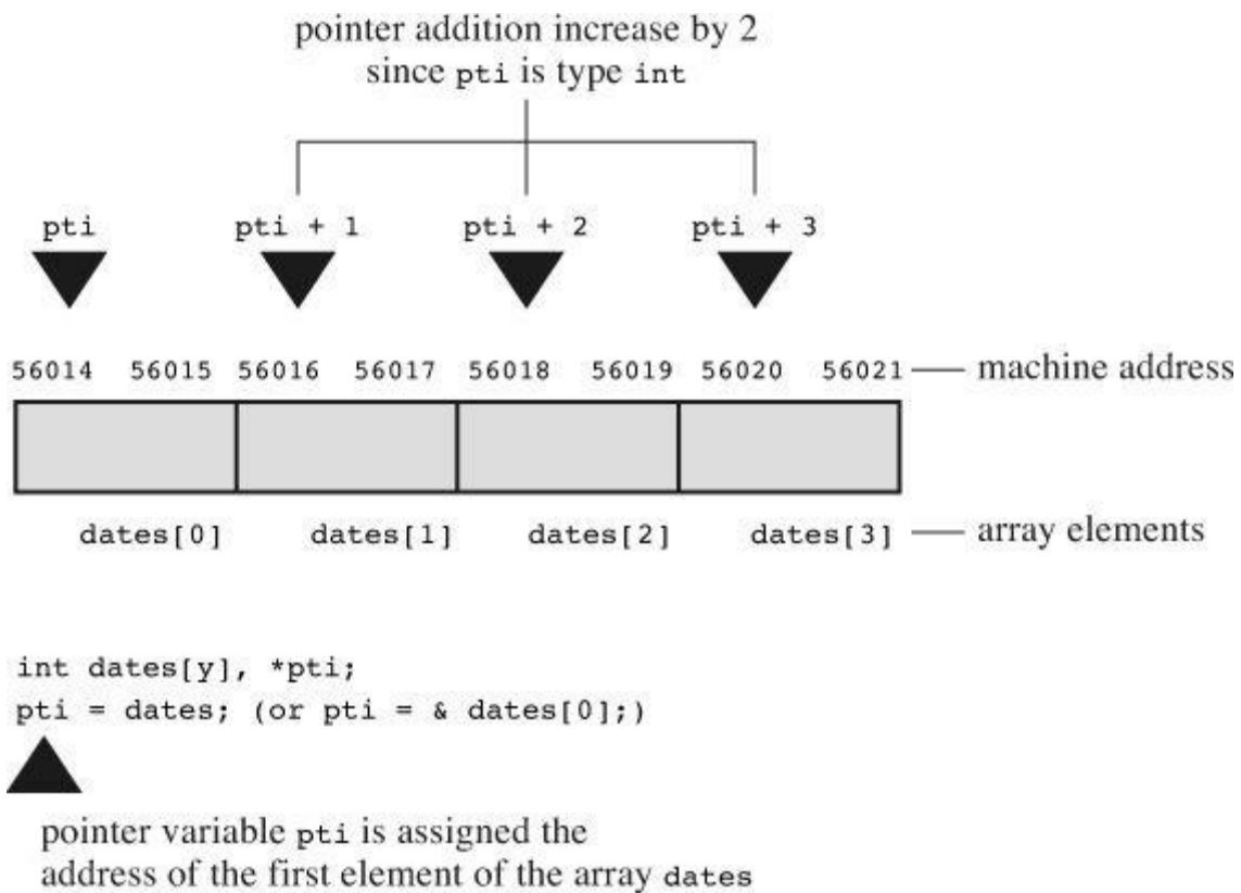
Figure 10.3 An array and pointer addition.
