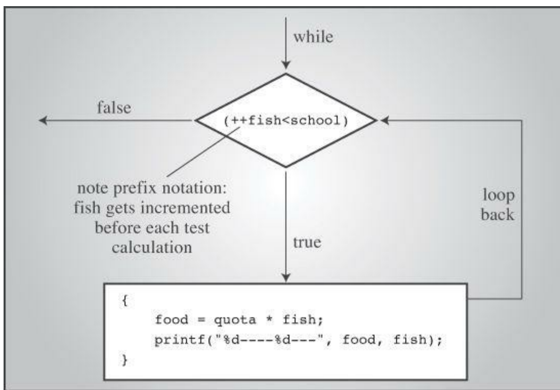
Figure 5.7 A while loop with a compound statement.
