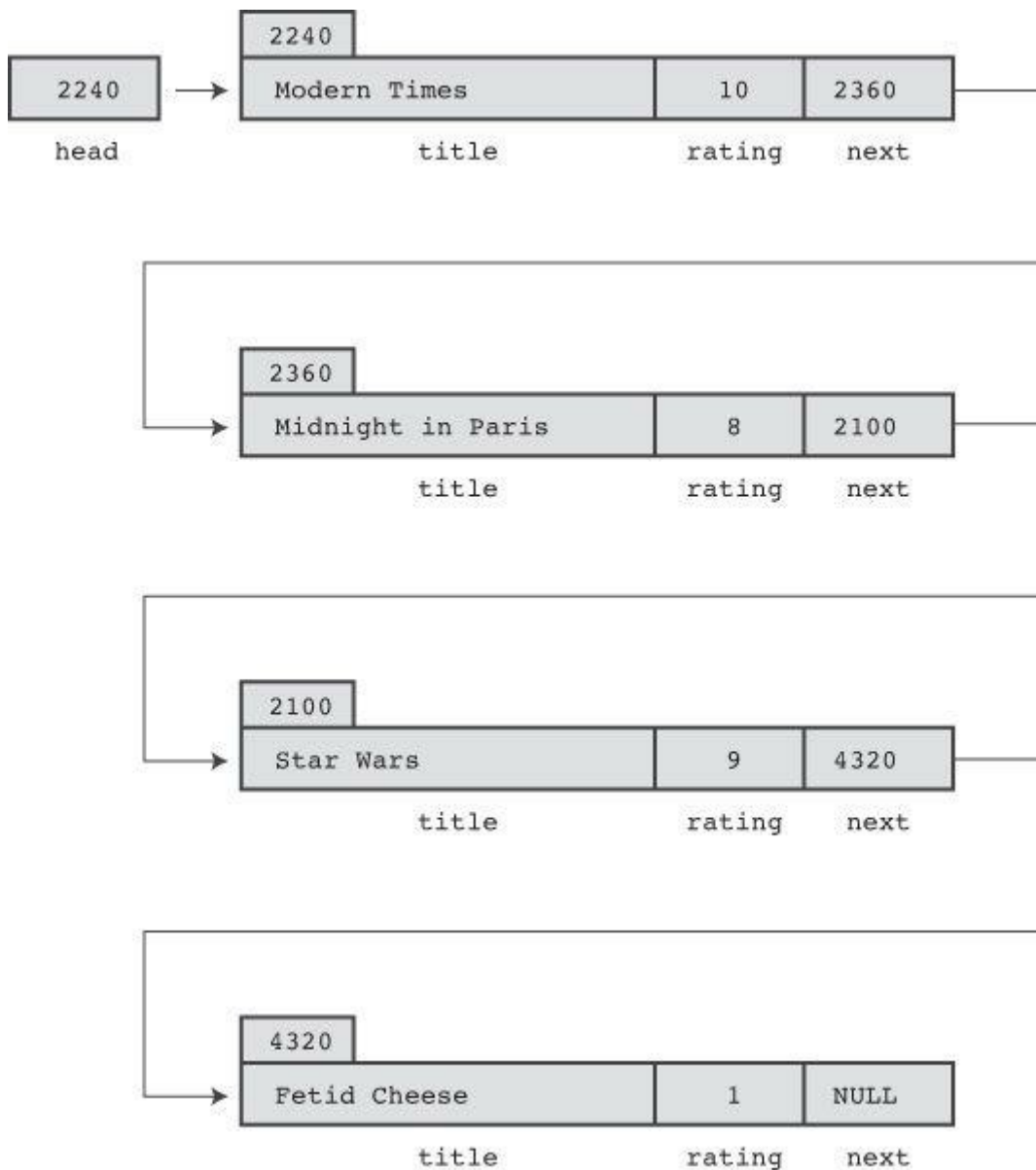
Figure 17.4 Linked list with several items.
