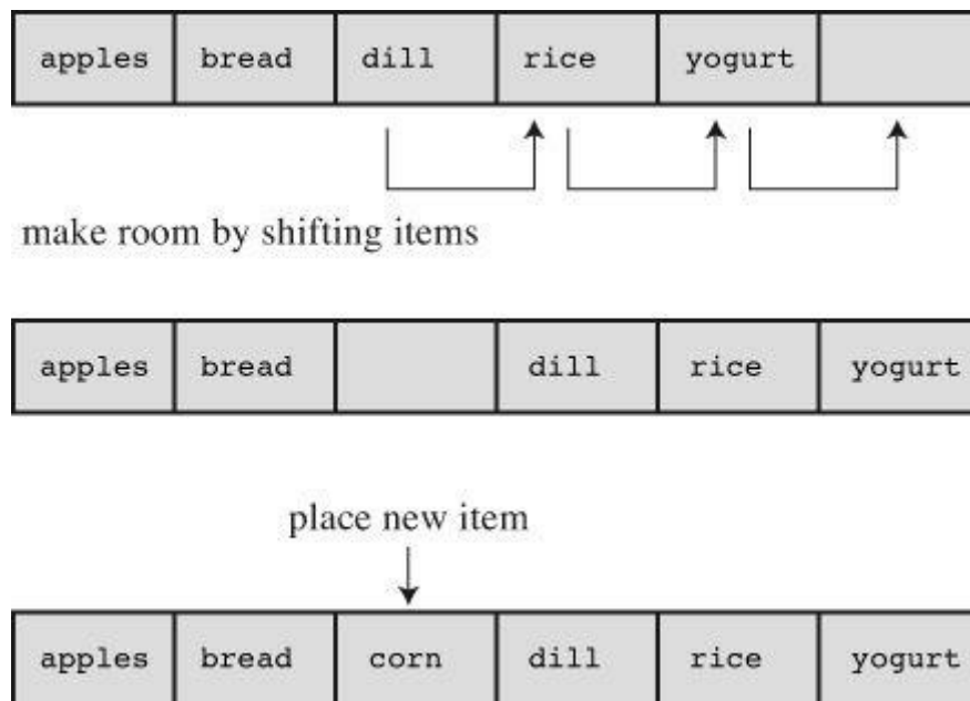
Figure 17.9 Inserting an element into an array.
