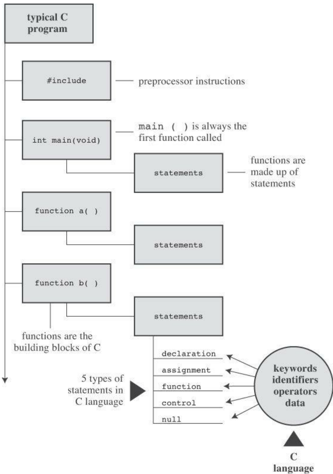
Figure 2.1 Anatomy of a C program.
