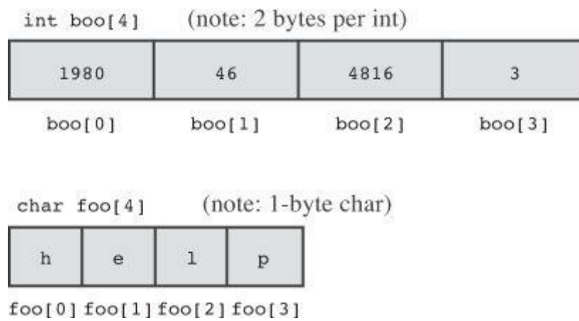
Figure 6.7 The char and int arrays in memory.
