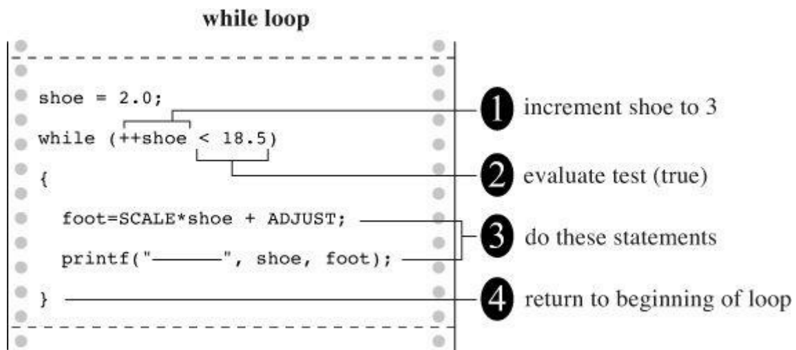
Figure 5.4 Through the loop once.
