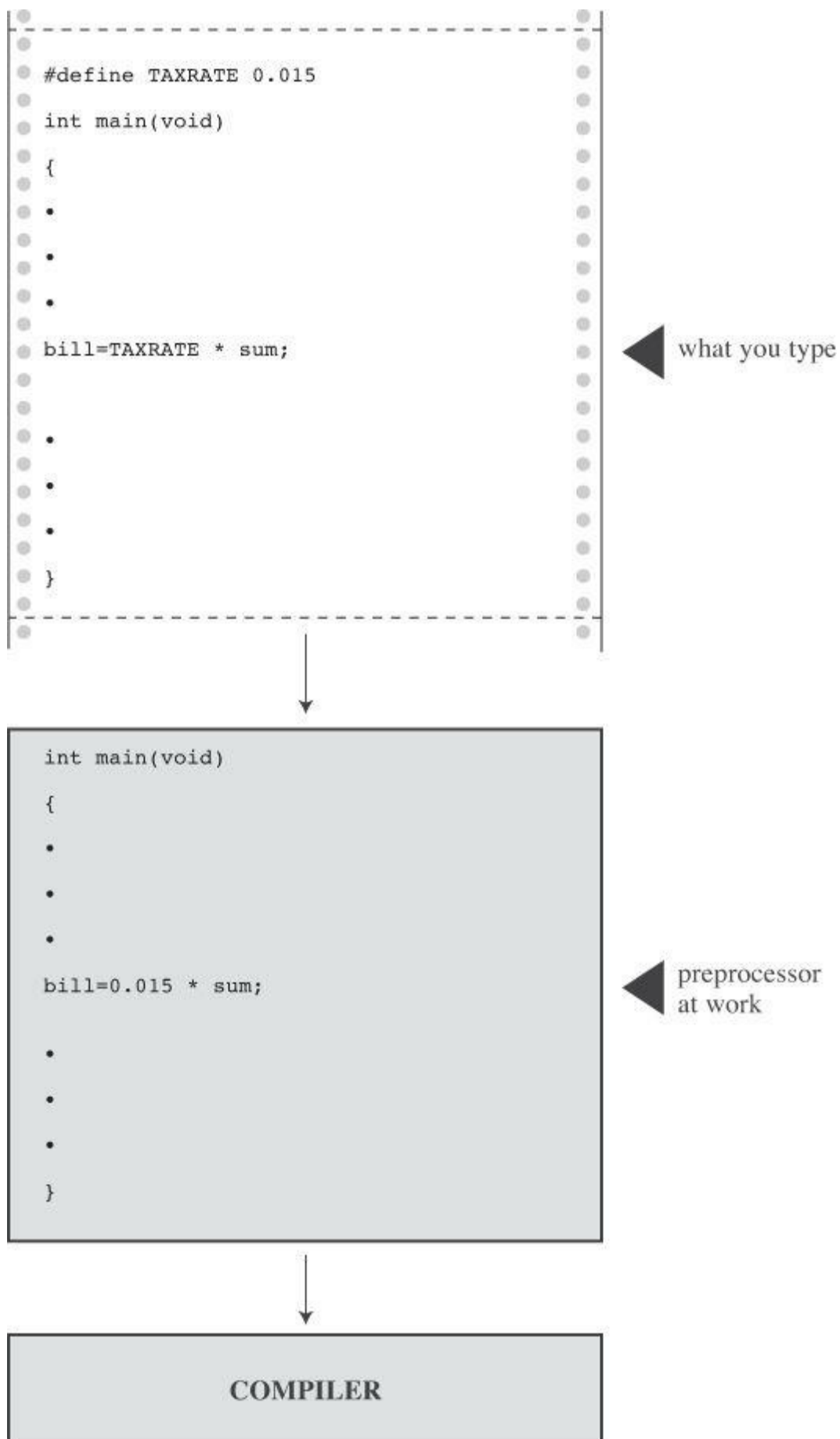
Figure 4.5 What you type versus what is compiled.
