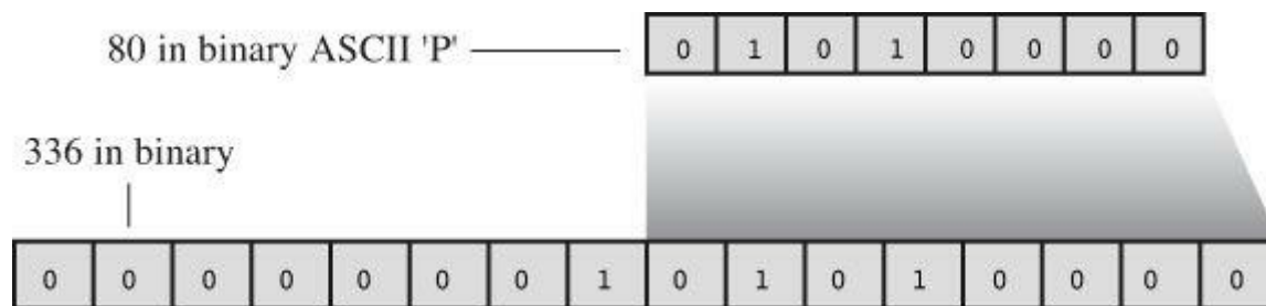
Figure 4.8 Reading 336 as a character.
