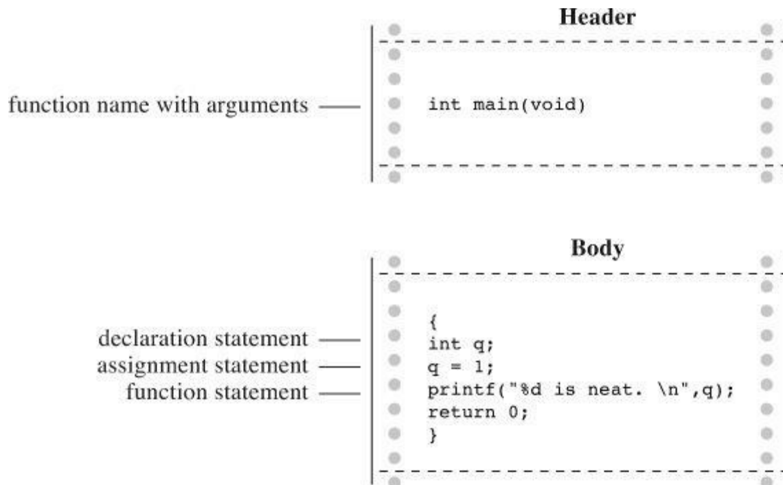
Figure 2.4 A function has a header and a body.
