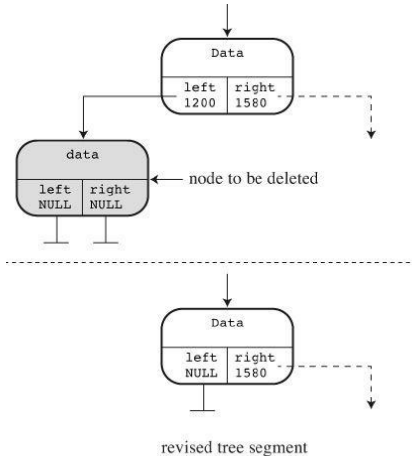
Figure 17.13 Deleting a leaf.
