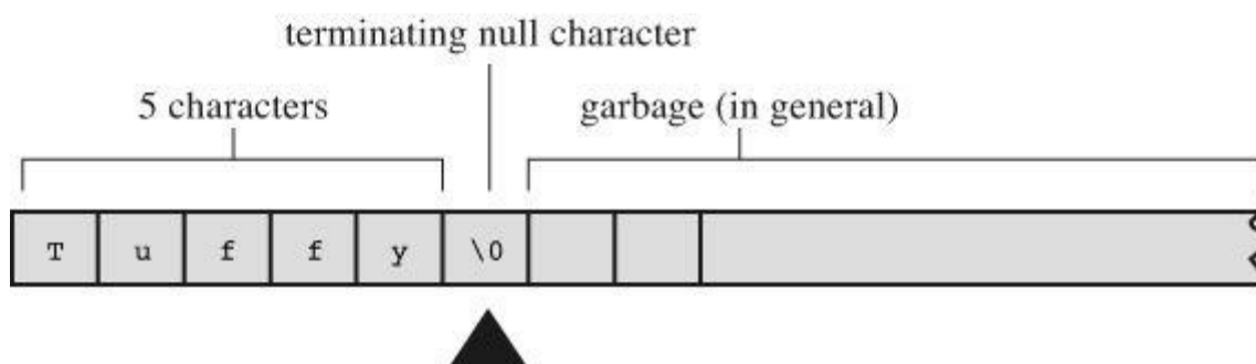
Figure 4.4 The strlen() function knows when to stop.
