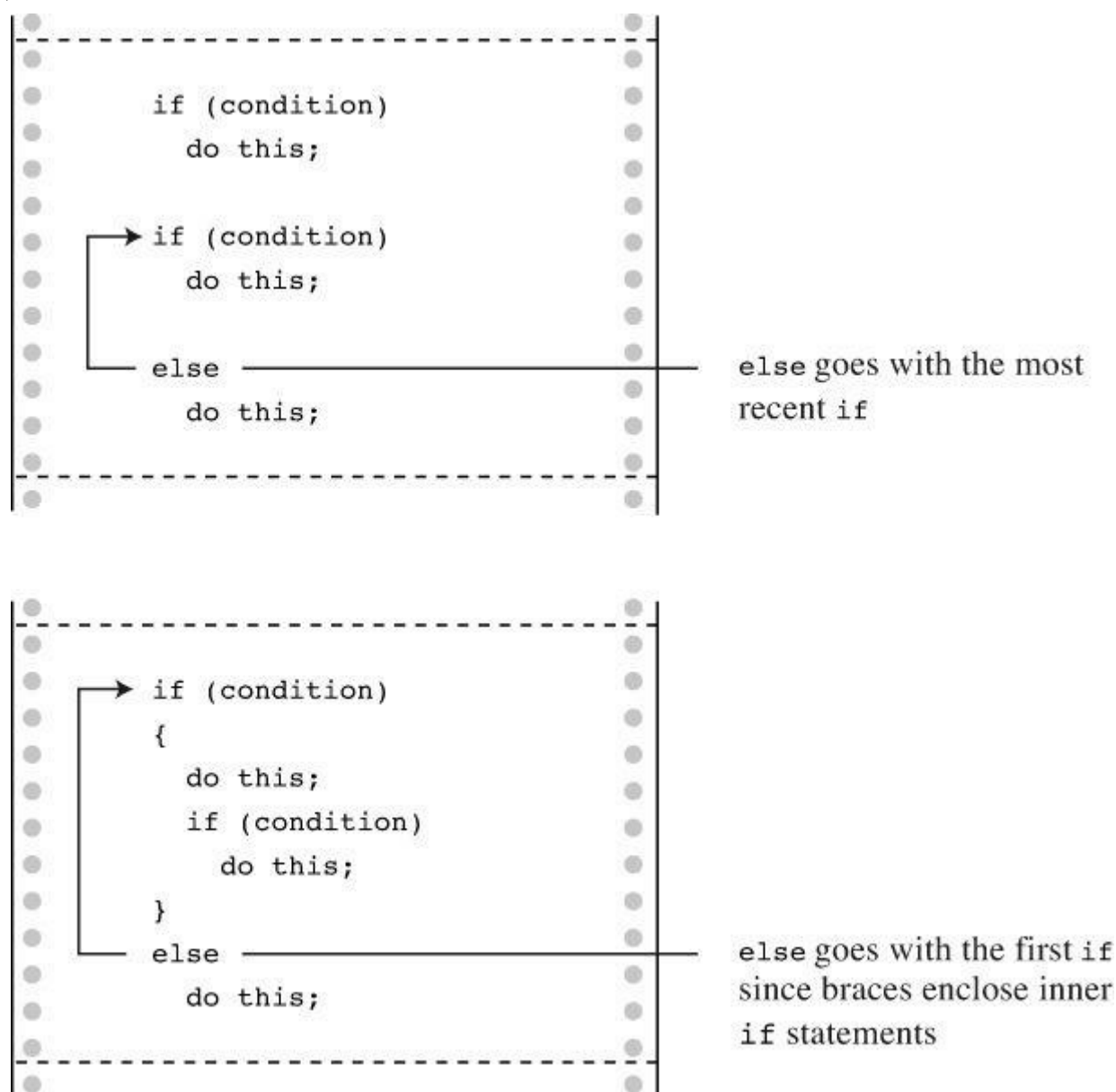
Figure 7.2 The rule for if else pairings.
