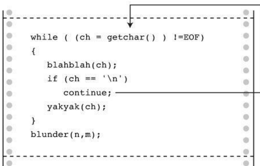
Figure 7.3 Comparing break and continue .
