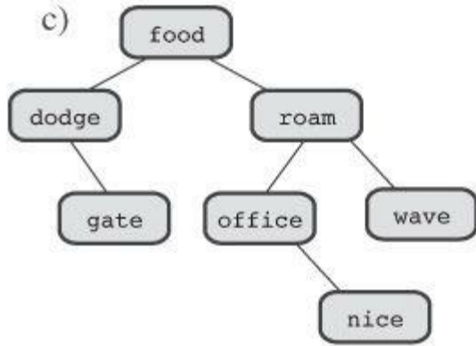
Figure A.1 Binary search tree of words.
