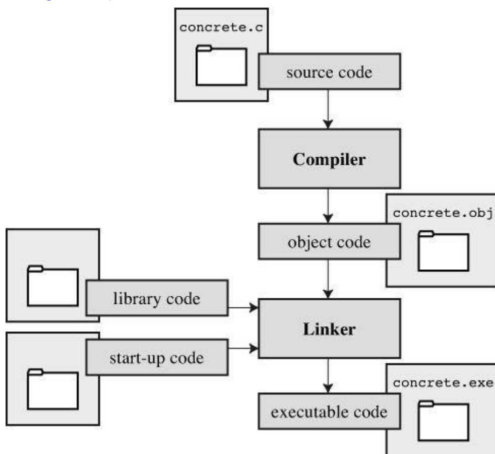
Figure 1.4 Compiler and linker.
