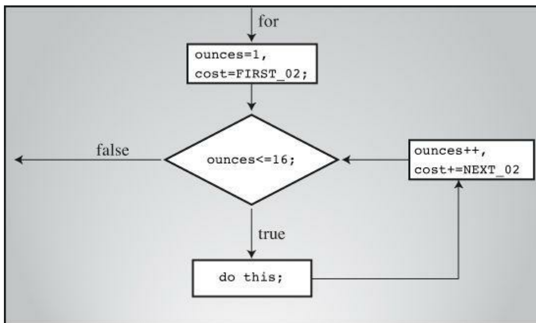
Figure 6.4 The comma operator and the for loop.
