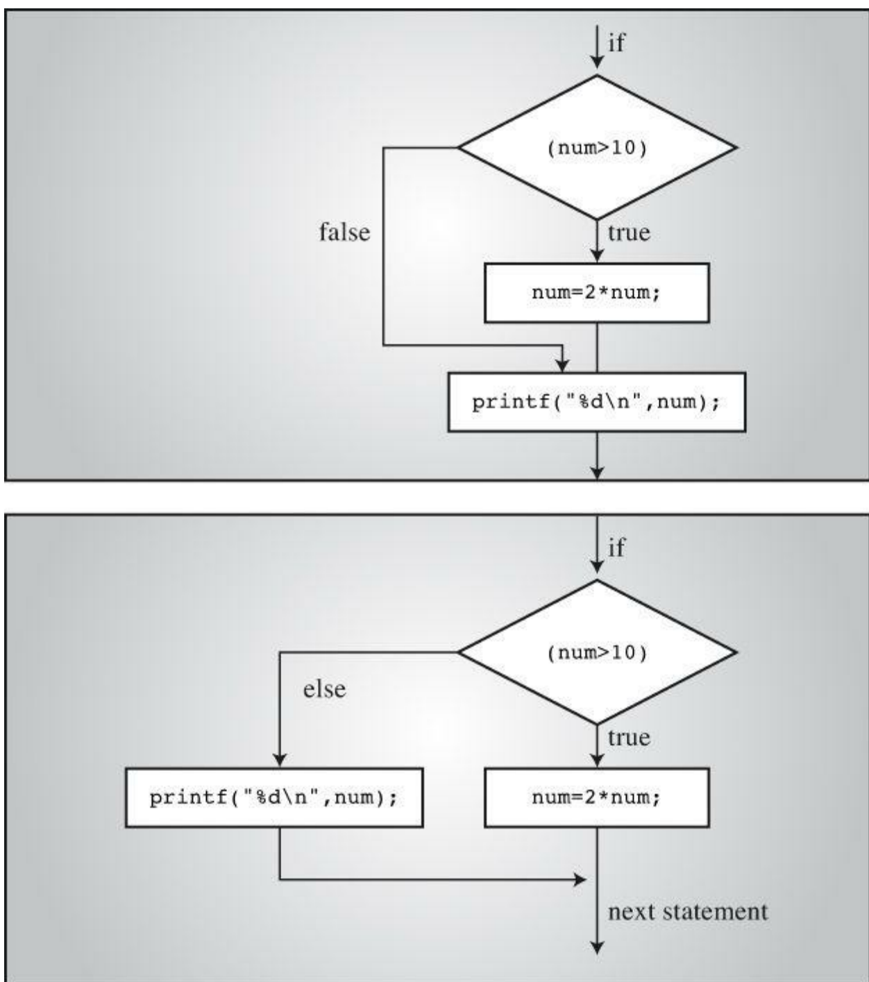
Figure 7.1 if versus if else.
