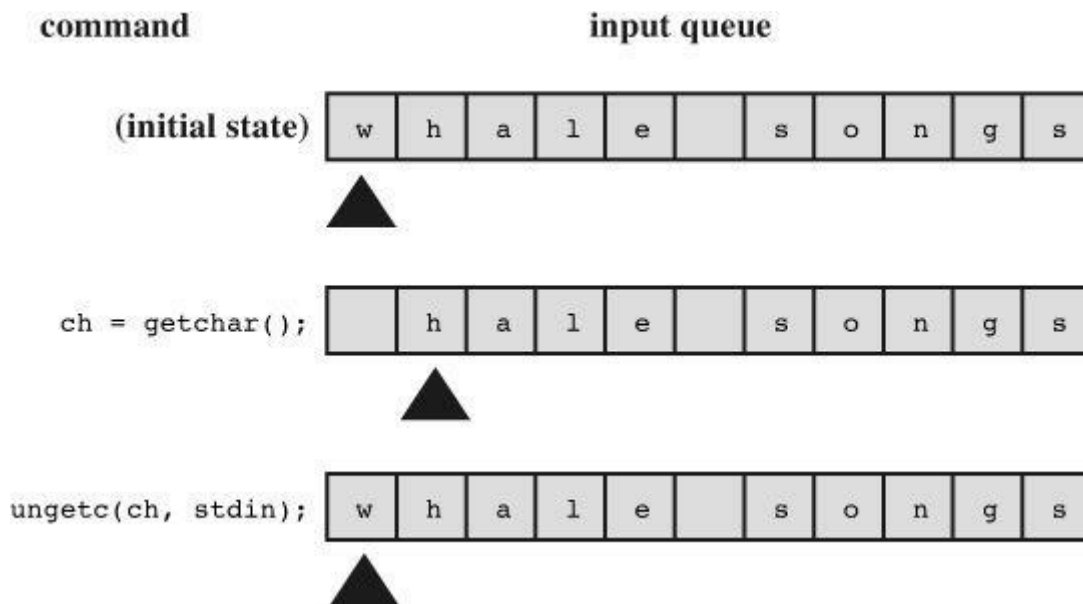
Figure 13.2 The ungetc() function.
