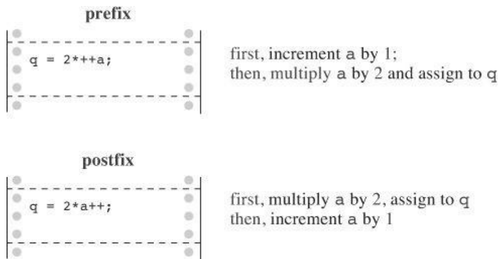
Figure 5.5 Prefix and postfix.
