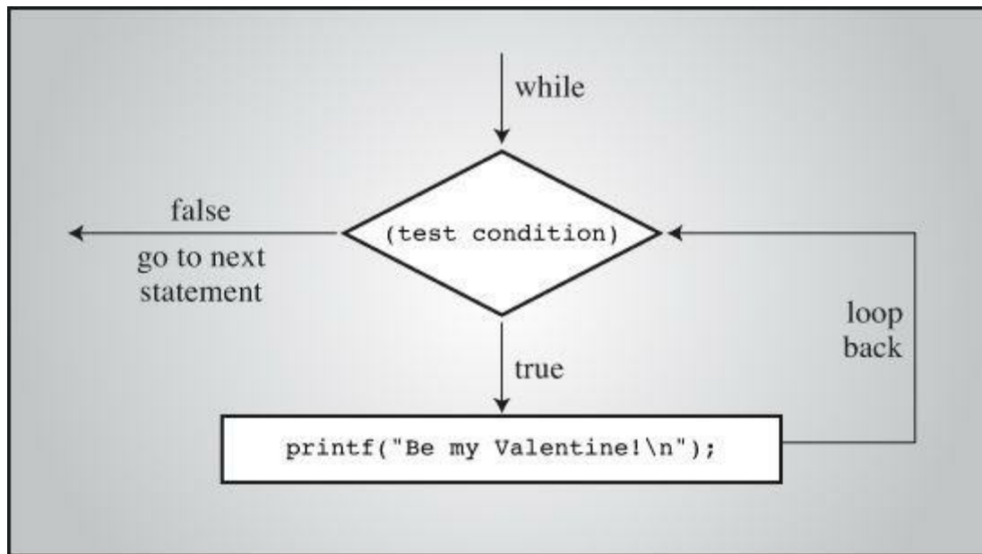
Figure 5.6 Structure of a simple while loop.
