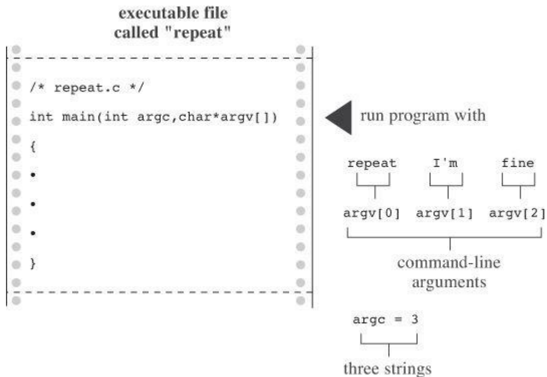
Figure 11.7 Command-line arguments.
