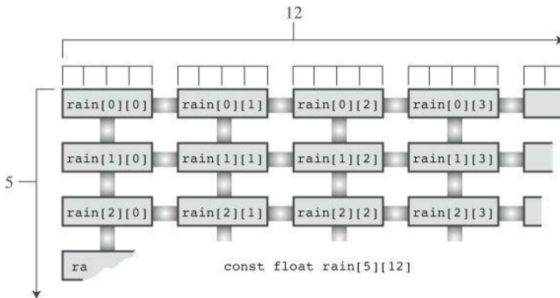
Figure 10.1 Two-dimensional array.
