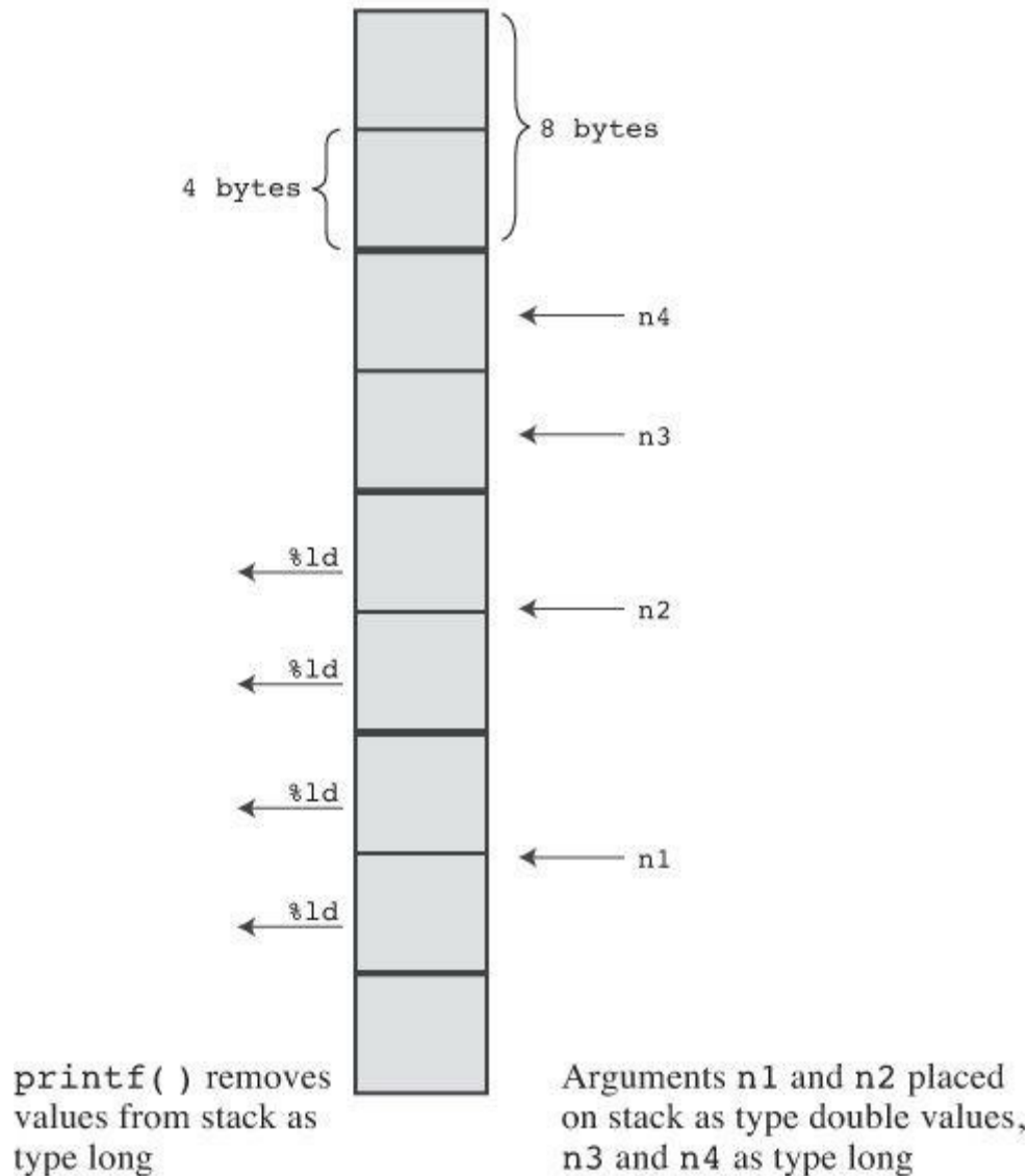
Figure 4.9 Passing arguments.
