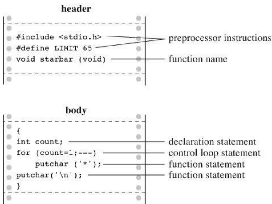
Figure 9.2 Structure of a simple function.
