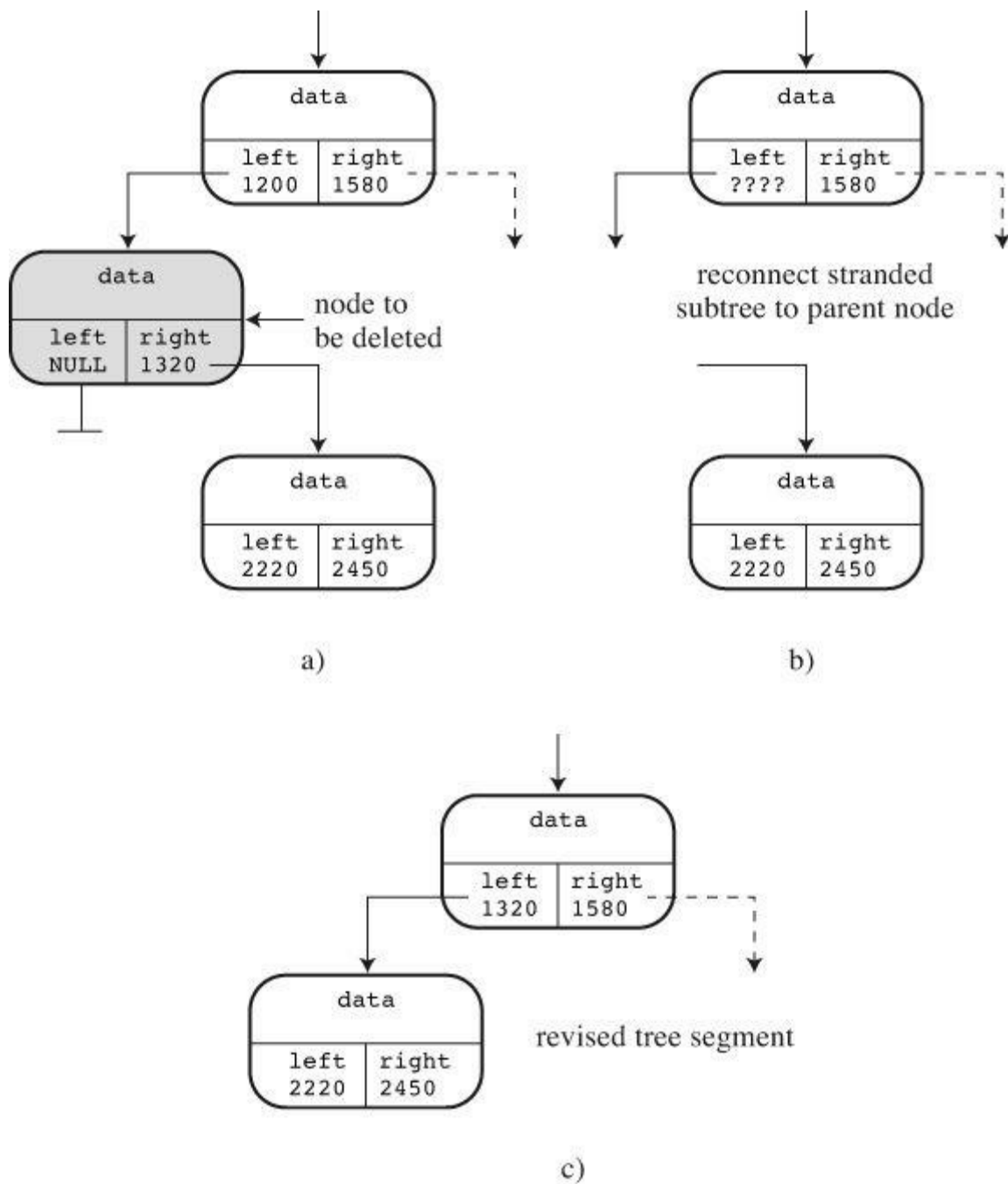
Figure 17.14 Deleting a one-child node.
