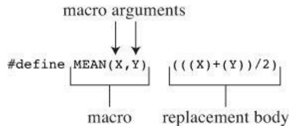
Figure 16.2 Parts of a function-like macro definition.
