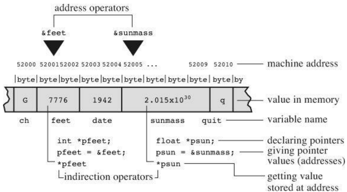
Figure 9.5 Declaring and using pointers.
