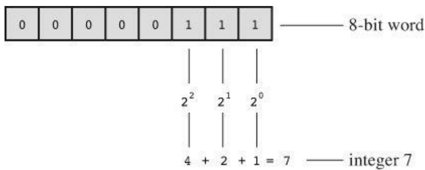
Figure 3.2 Storing the integer 7 using a binary code.
