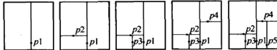
图 12-53 平面由 2-d 树在插入 p_1 = (53, 14) , p_2 = (27, 28) , p_3 = (30, 11) , p_4 = (67, 51) , p_5 = (70, 3) 后所得到的划分
